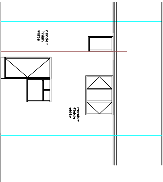
PROPOSED REAR VIEW 1: 100
