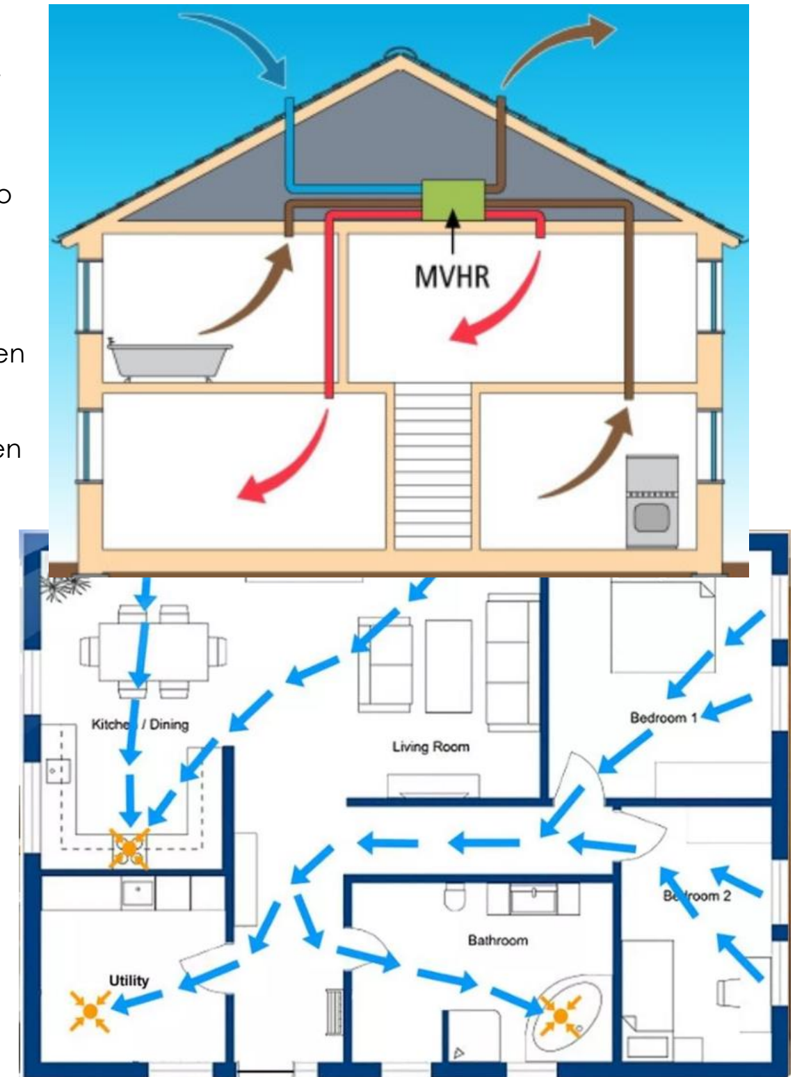
Figure 12: Depiction of air paths within a dwelling using an MVHR system
