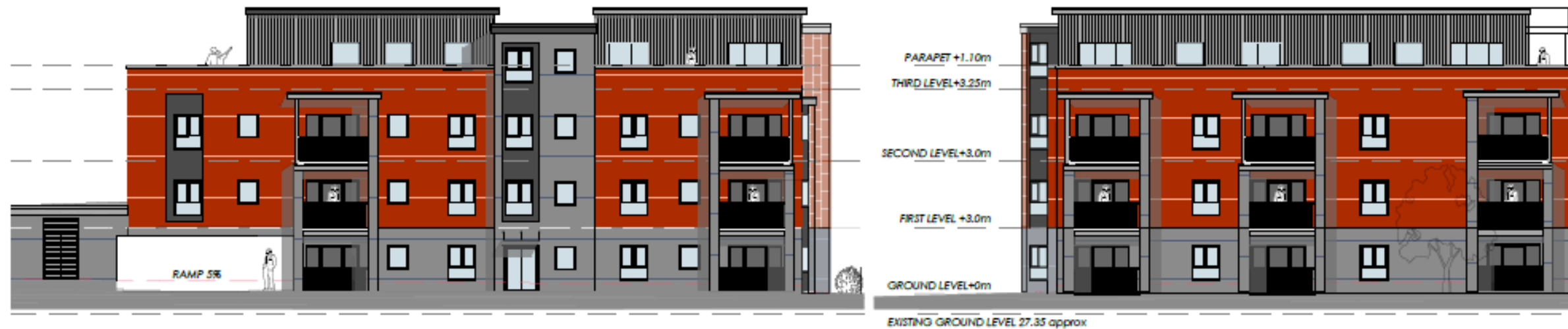
FRONT ELEVATION (Albany Road )
