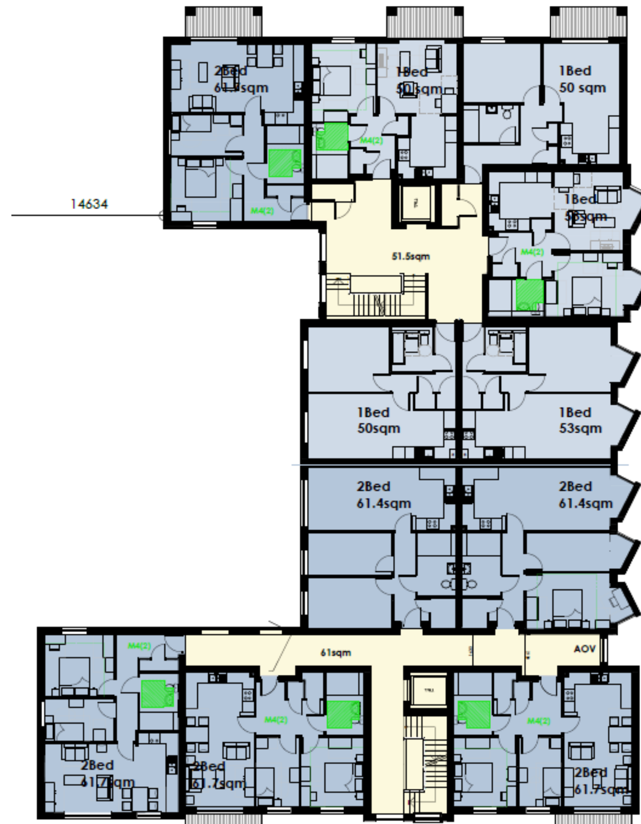
Figure 6: Architectural drawings – Second Floor Plan
