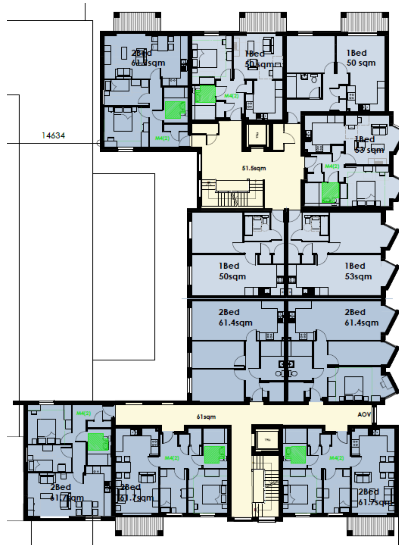
Figure 5: Architectural drawings – First Floor Plan
