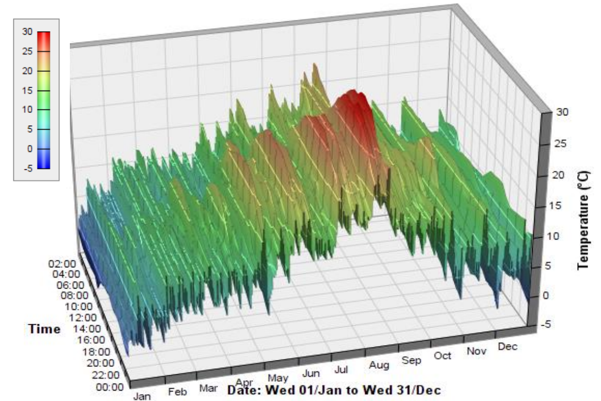
Figure 2: Annual dry-bulb temperature graph of modelled weather file
