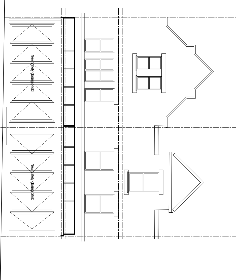
SHOP FRONT ELEVATION 1:100@A4
