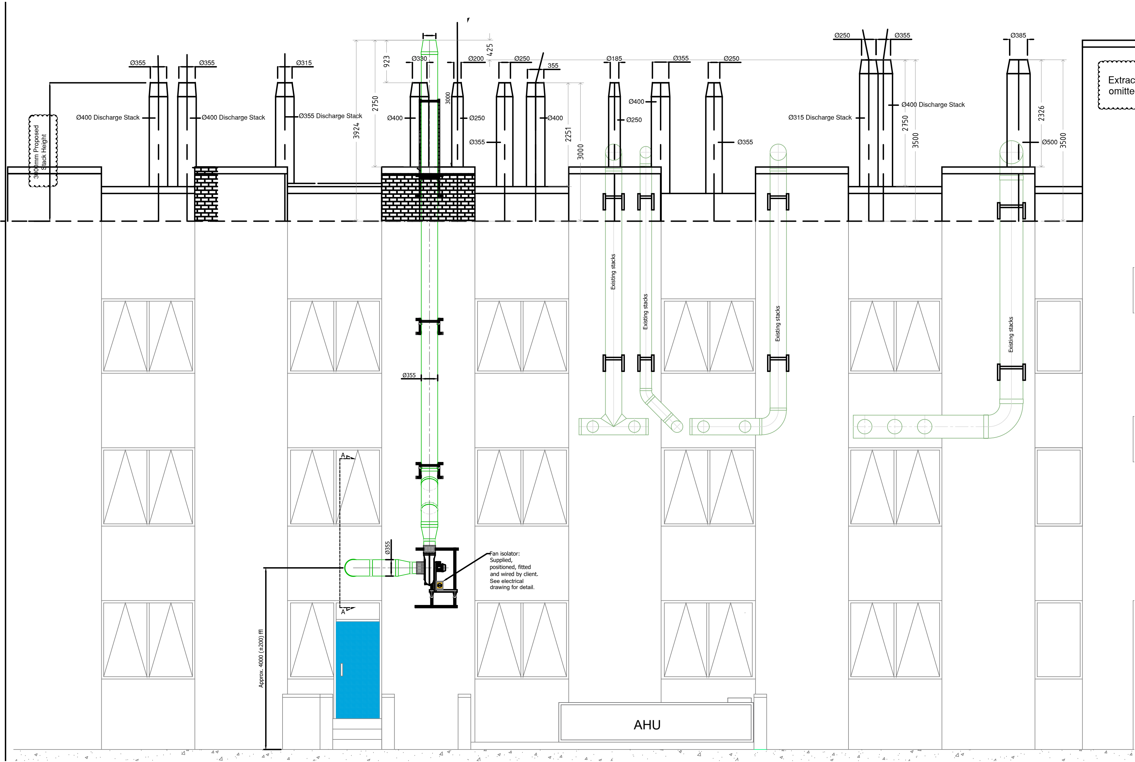
Proposed Elevation
