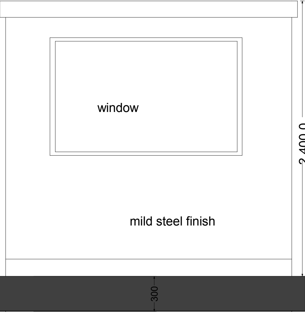
West elevation
