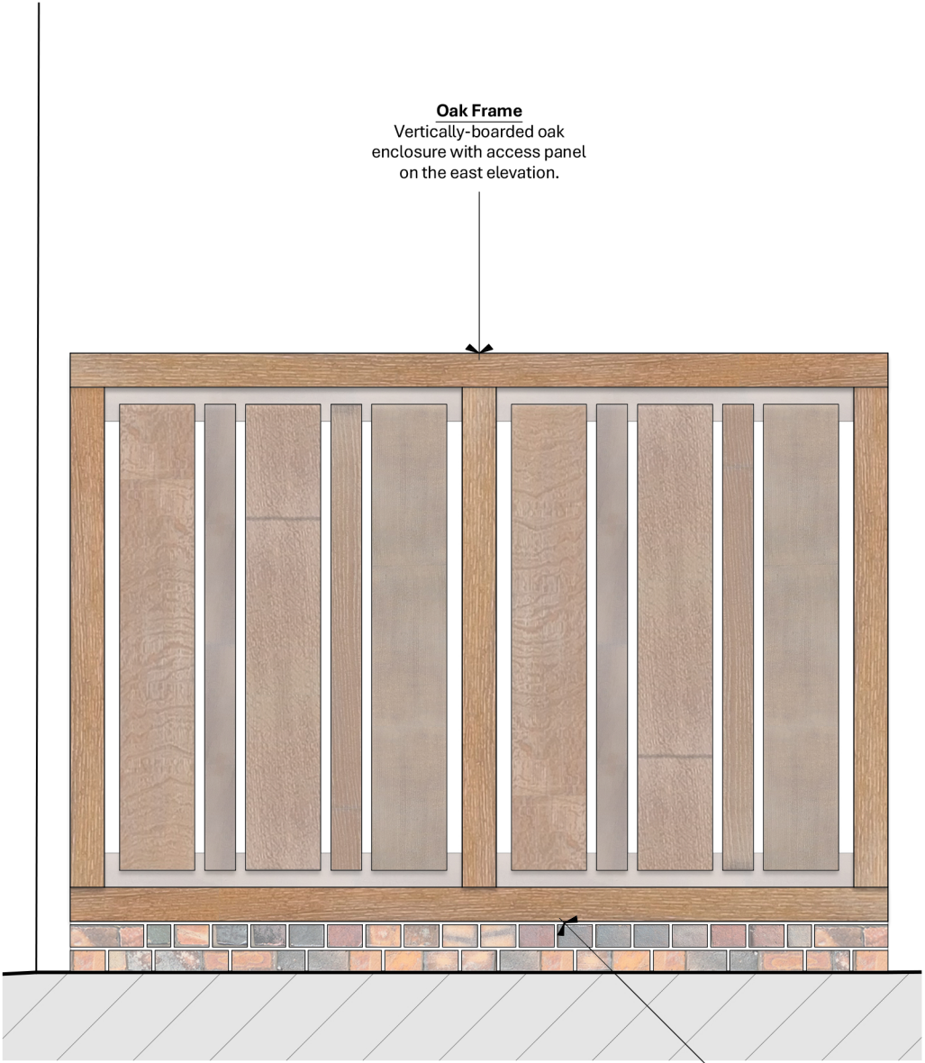
West Elevation ASHP Enclosure
