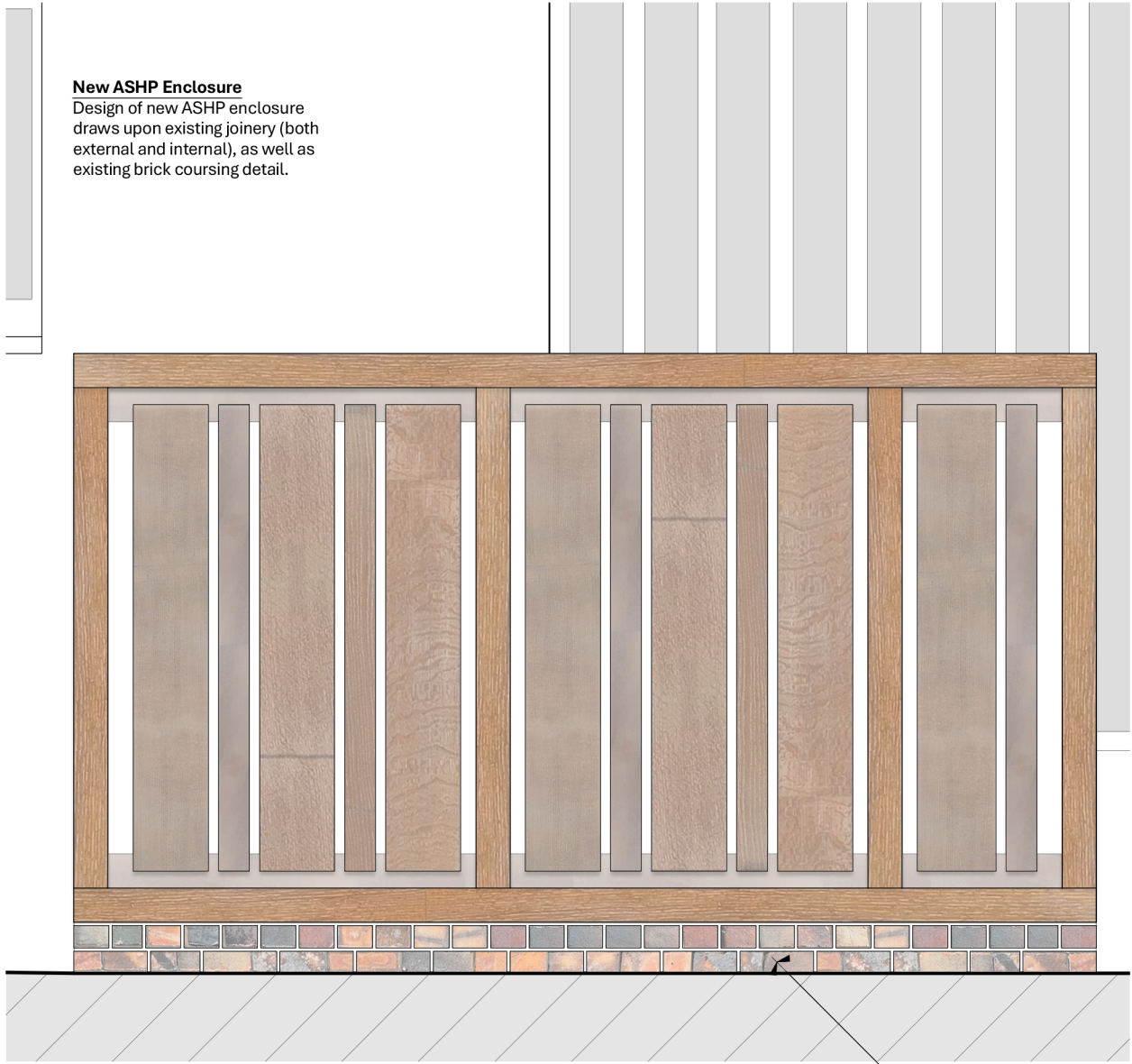
South Elevation ASHP Enclosure
