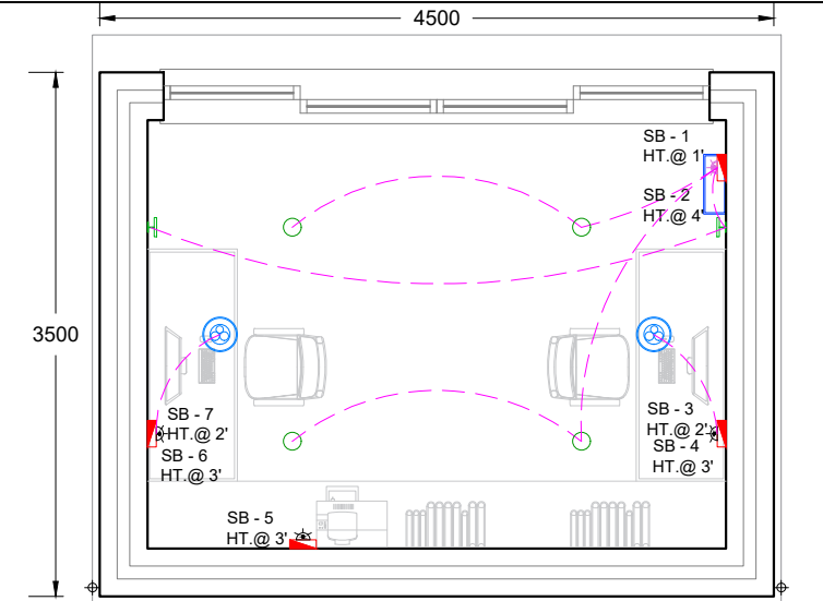
PROPOSED ELECTRICAL CONDUIT PLAN
