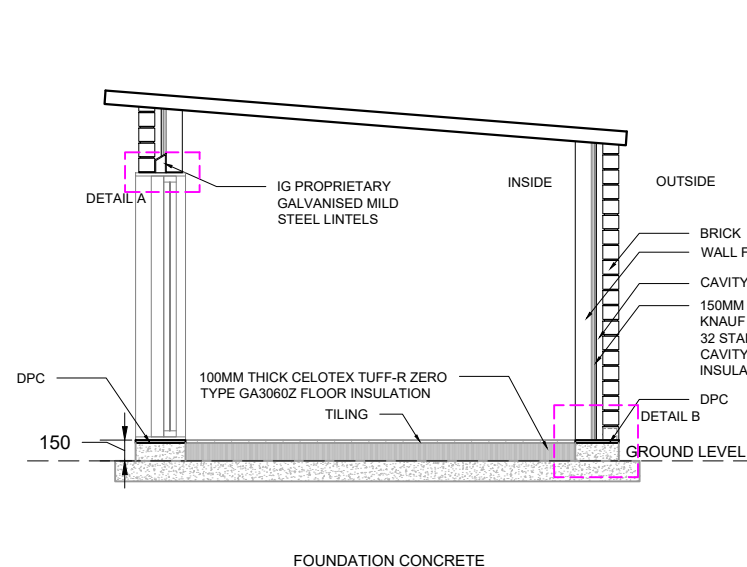
WALL SECTION
