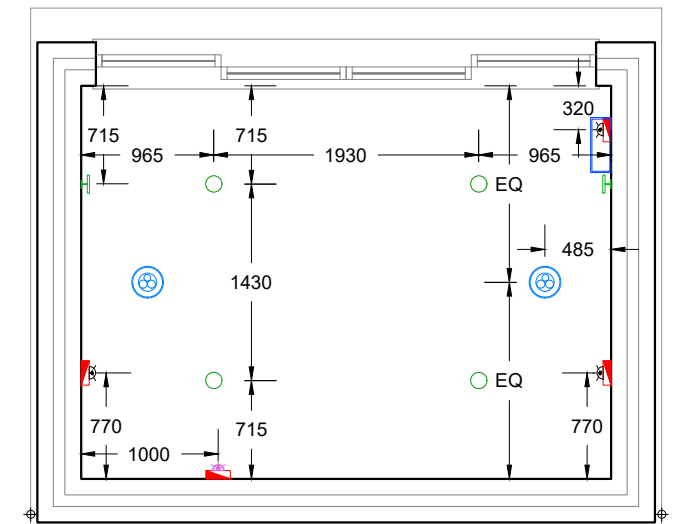
PROPOSED ELECTRICAL DIMENSION PLAN
