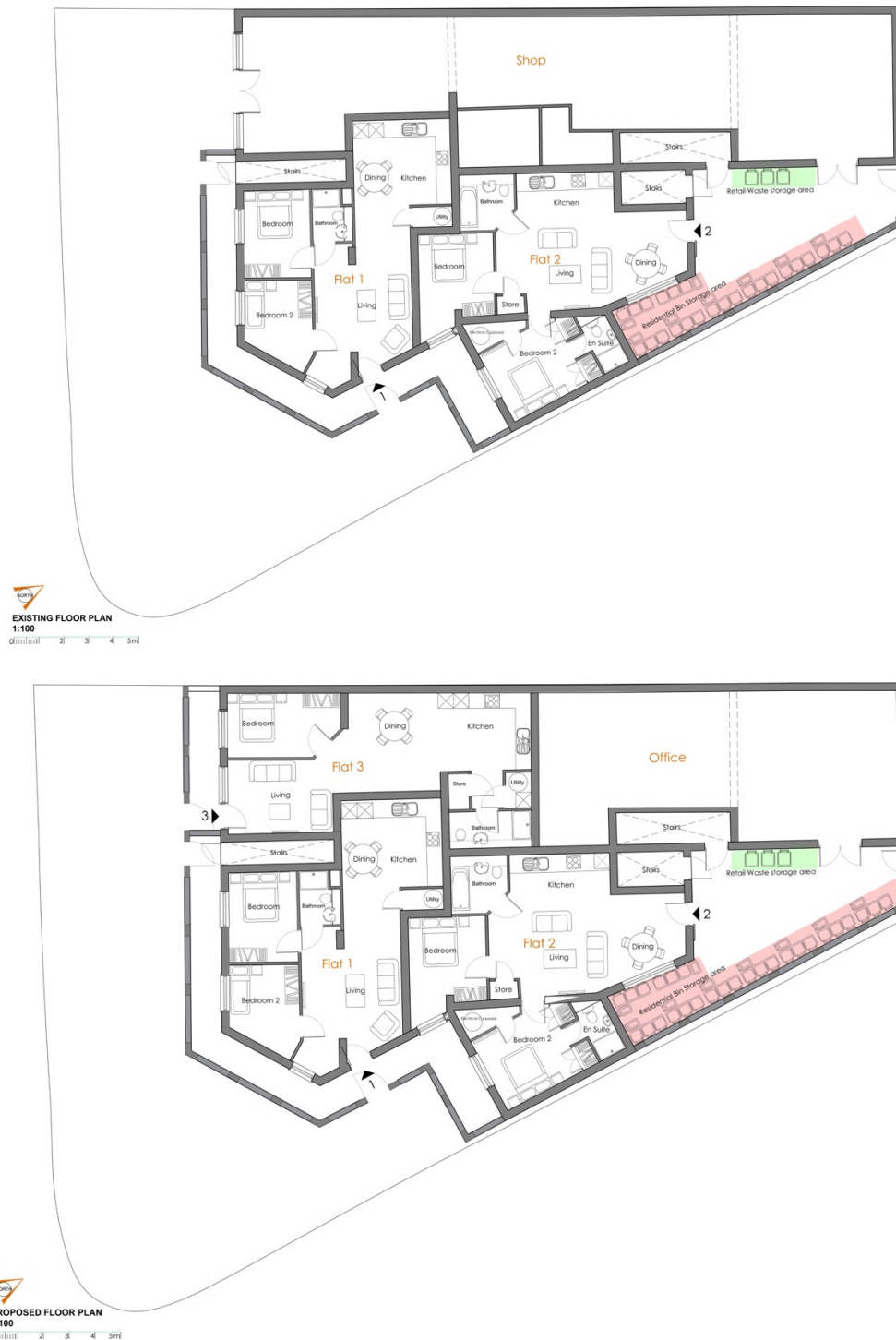
Fig 2: Existing and proposed ground floor plans.
