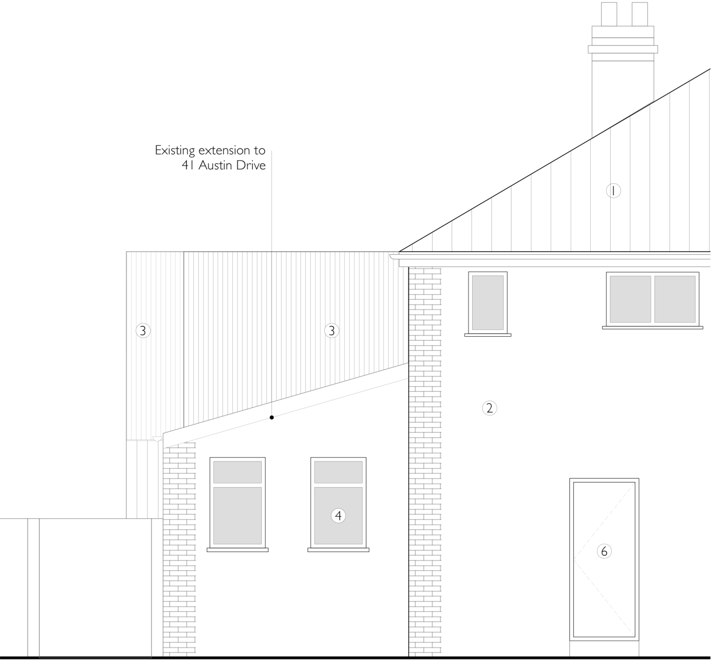
022.01 - Proposed East Elevation
