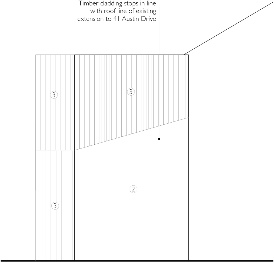
022.02 - Proposed East Elevation 02
