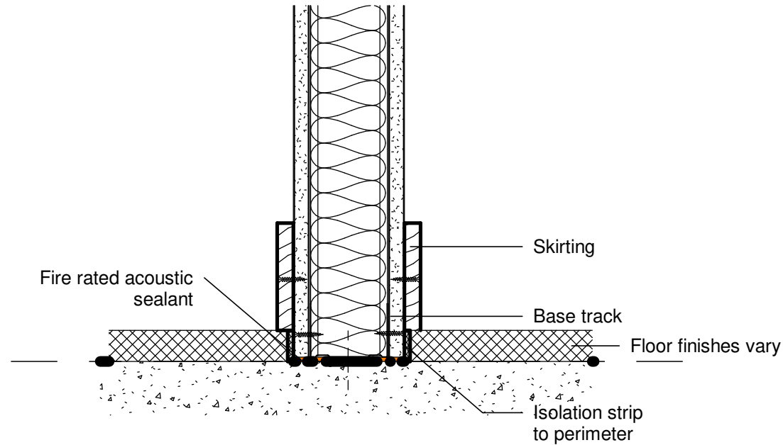
1 Typical head & base detail - section 1:5
