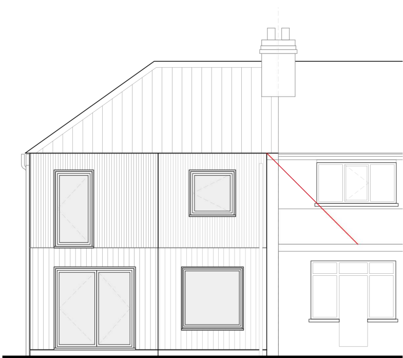
03 - Proposed rear elevation showing 45 degree line in elevation
