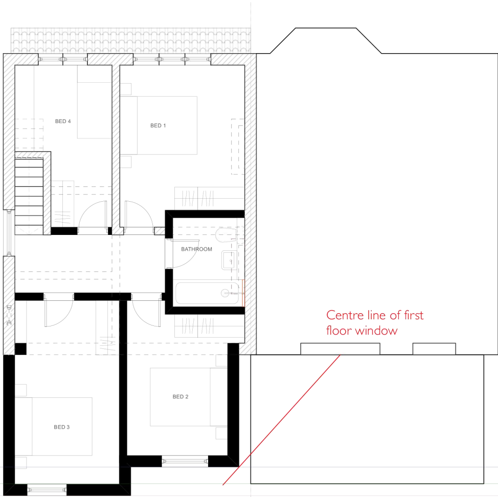
02 - Proposed First Floor Plan
