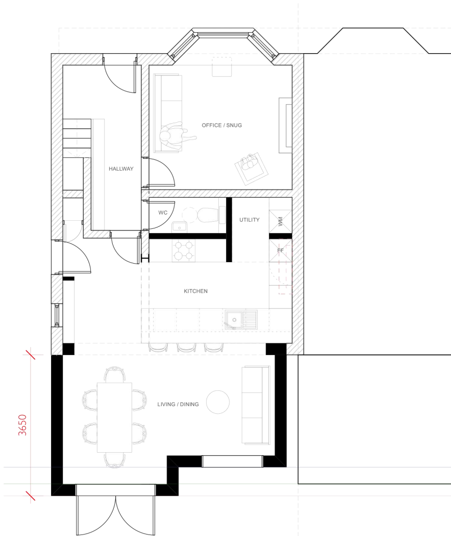
01 - Proposed Ground Floor Plan
