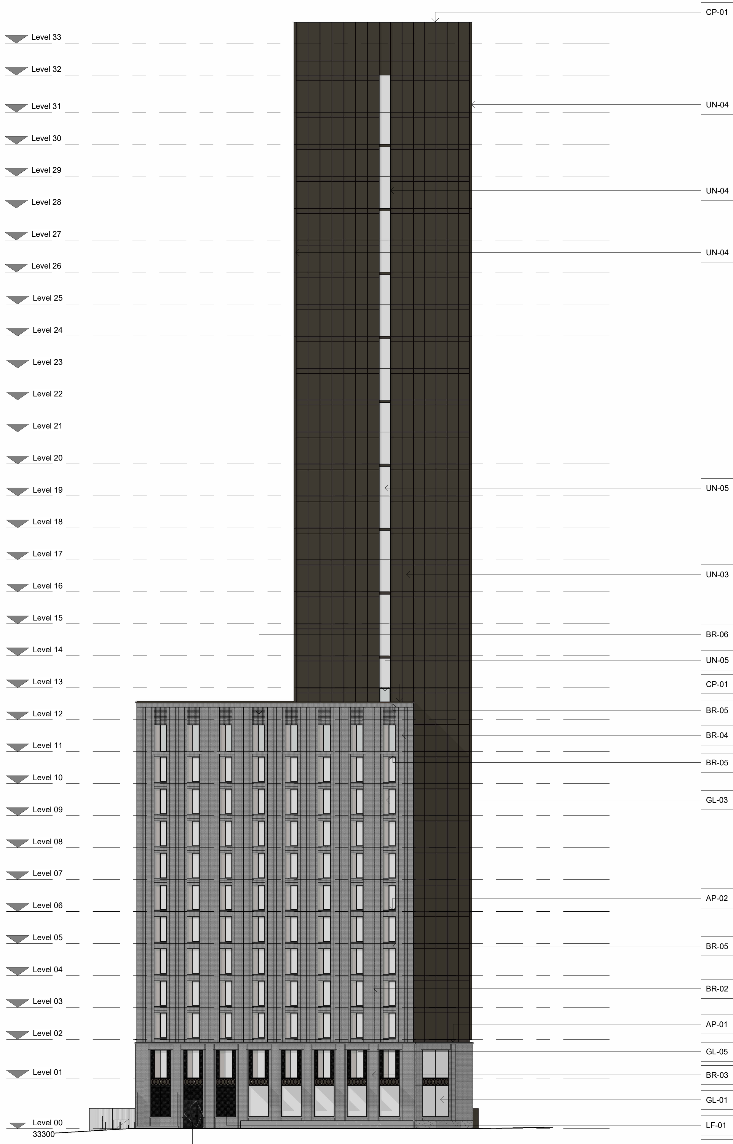
2: GA Elevation - West 1 : 200
