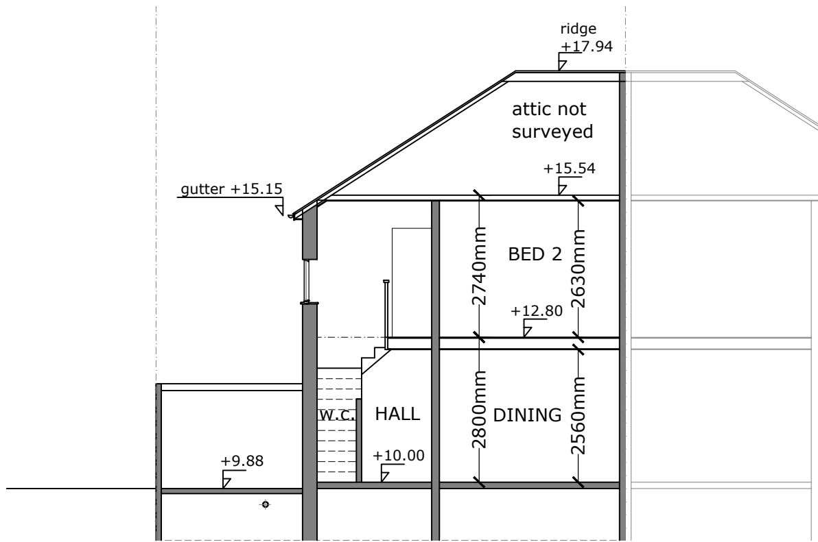
assumed drain depth assumed foundation depth CROSS SECTION
