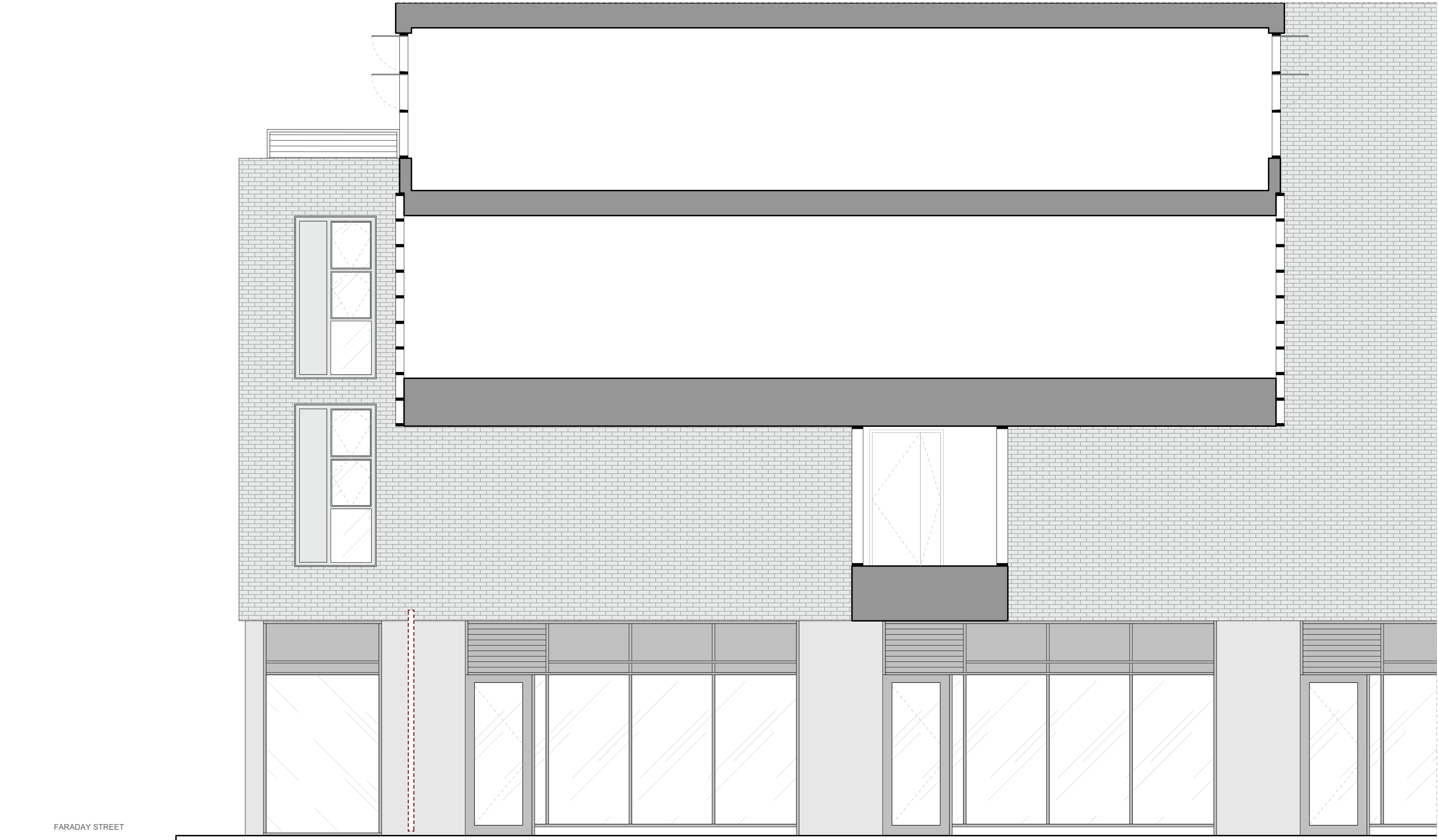
1 BUILDING PASSAGE - EXISTING SECTION Scale: 1:50
