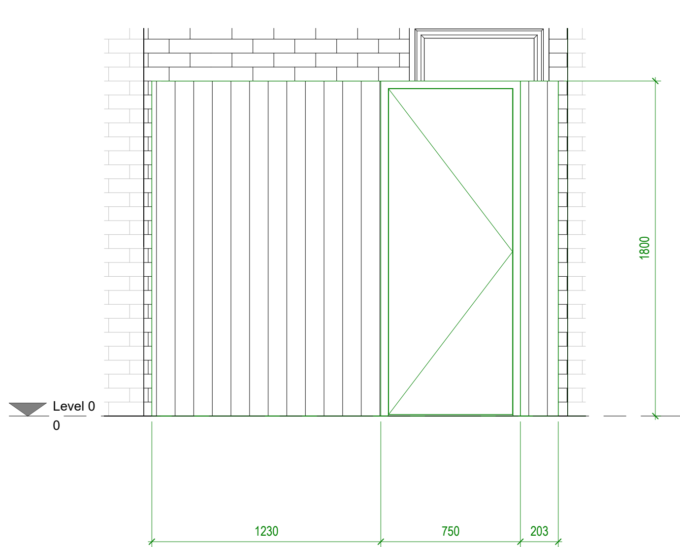
1 Bin Store Elevation 1 1 : 20
