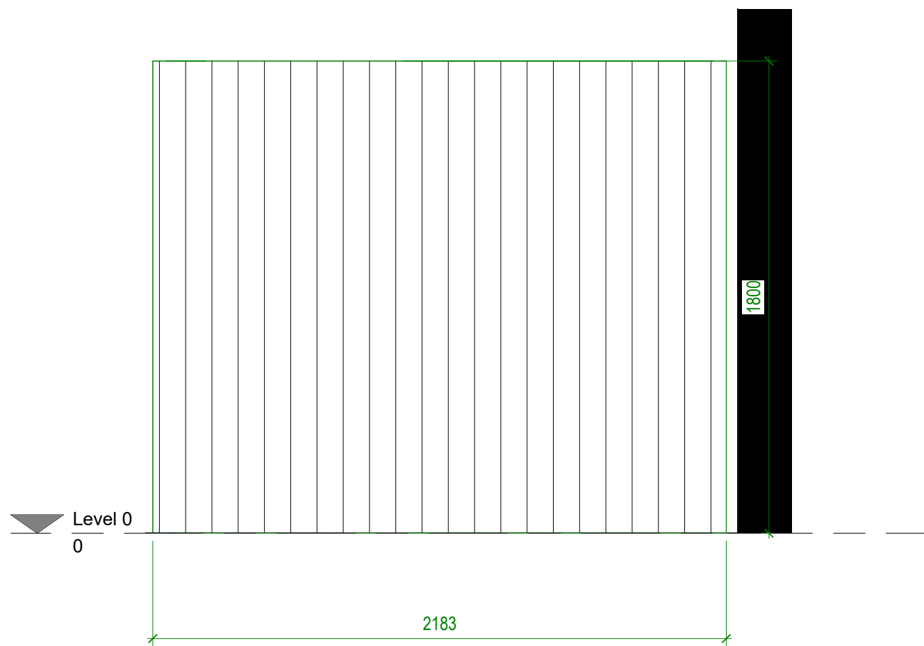
3 Bin Store Elevation 3 1 : 20
