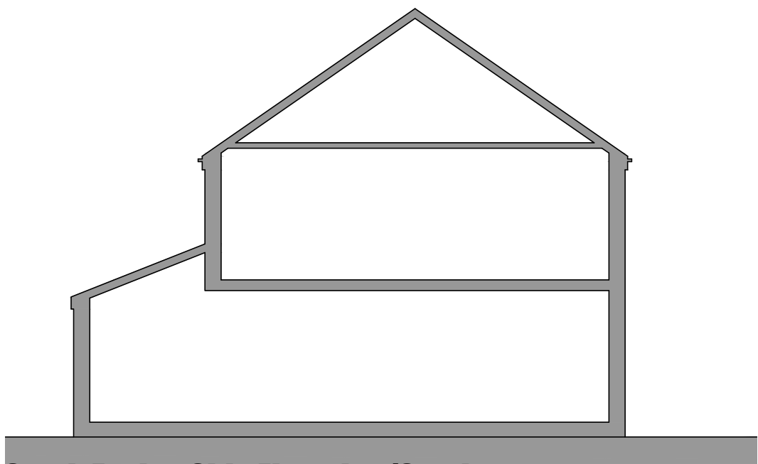
South Facing Side Elevation/Section
