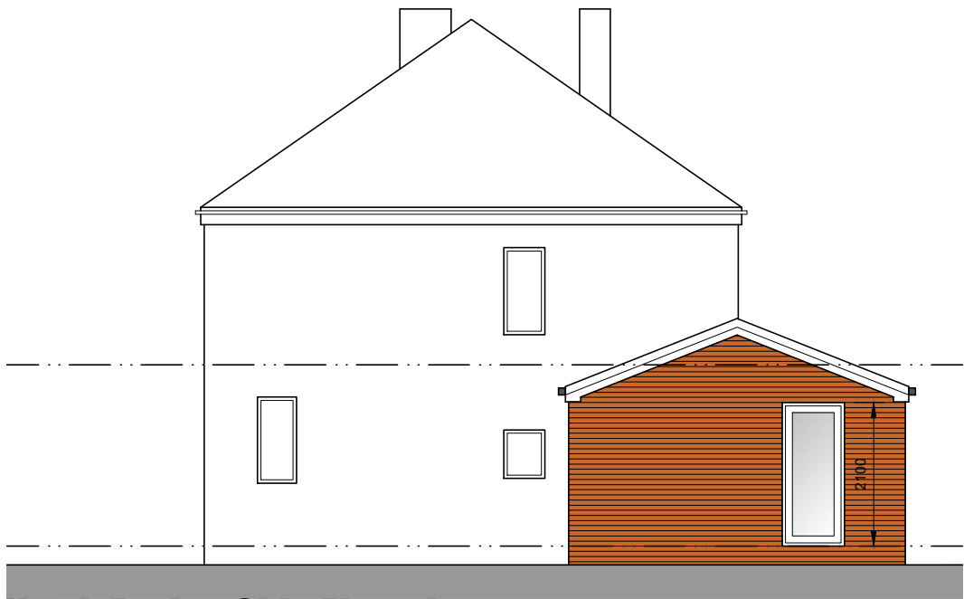
North Facing Side Elevation
