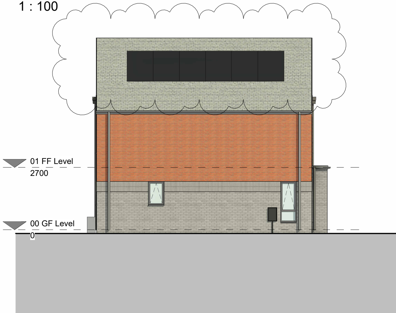
Left Elevation 1 : 100
