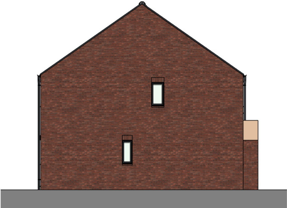
Left Elevation 1 : 100
