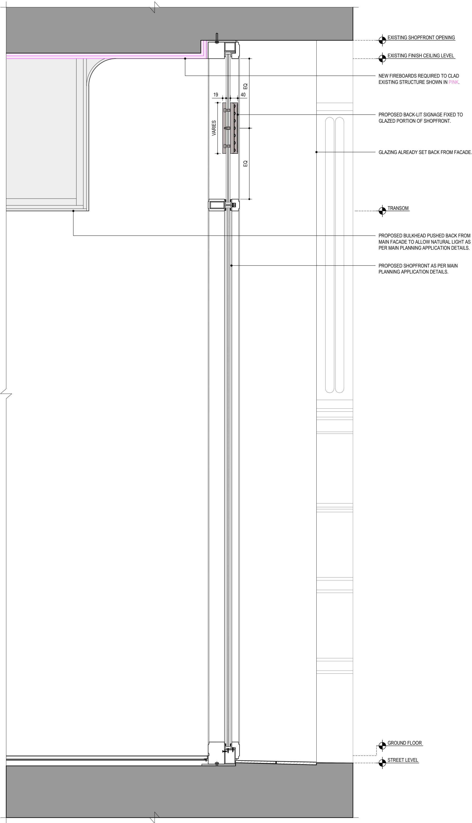
2 PROPOSED SHOPFRONT SECTION SCALE 1:10@A1; 1:20@A3
