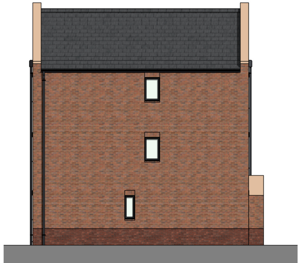
Left Elevation 1 : 100
