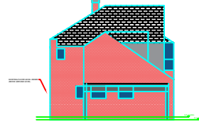
East Elevation
