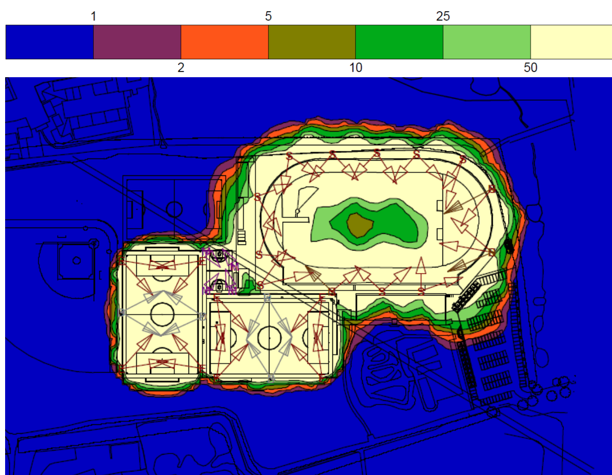
Figure 6 – Floodlighting Illuminance (Lux)
