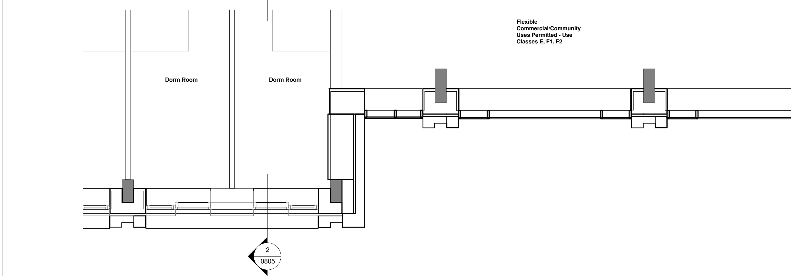
3 Bay Study Plan - BZ - Level 01
