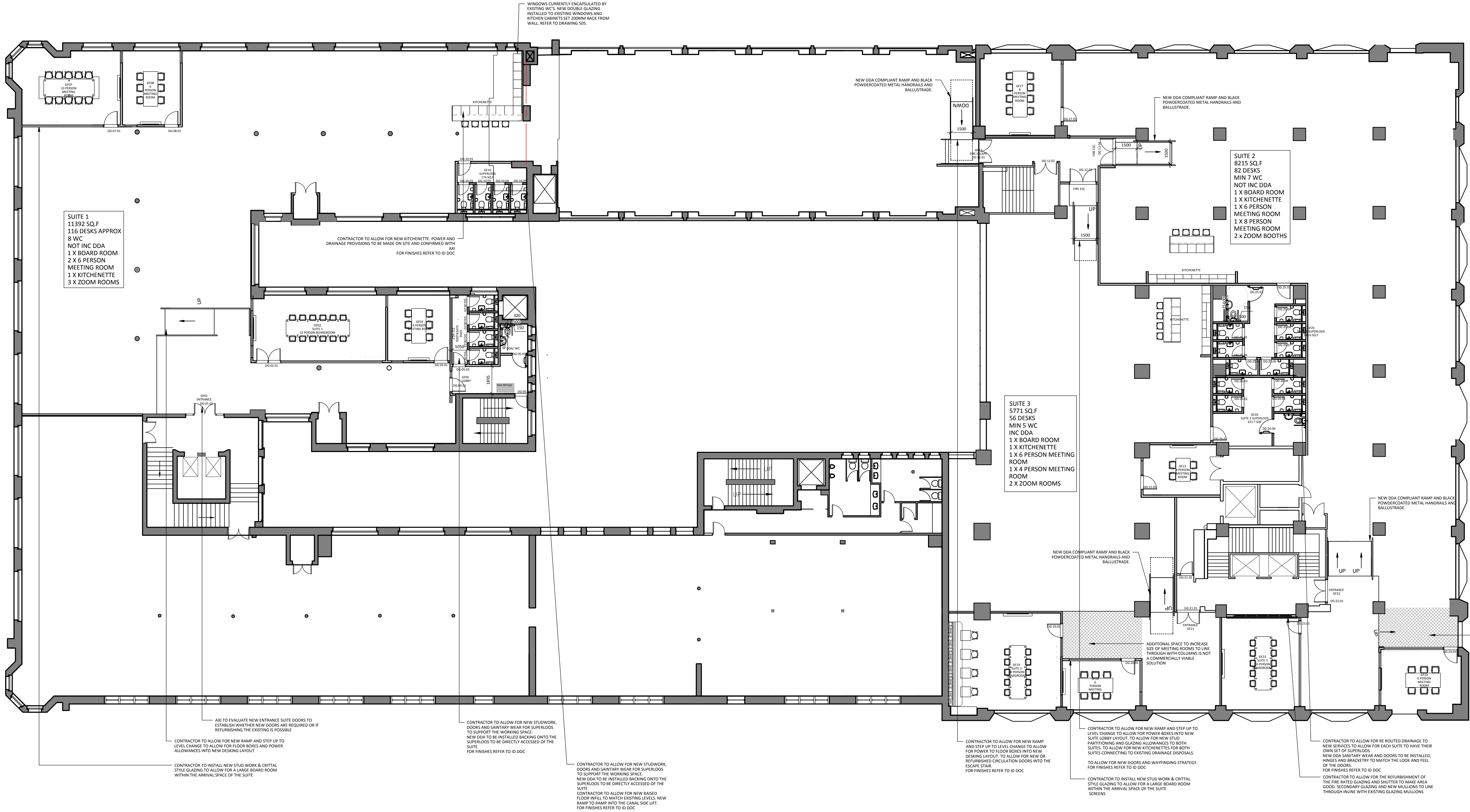
01 200 PROPOSED SECOND FLOOR CHURCHGATE & THIRD FLOOR LEE HOUSE PLAN SCALE - NTS @ A1 PLAN
