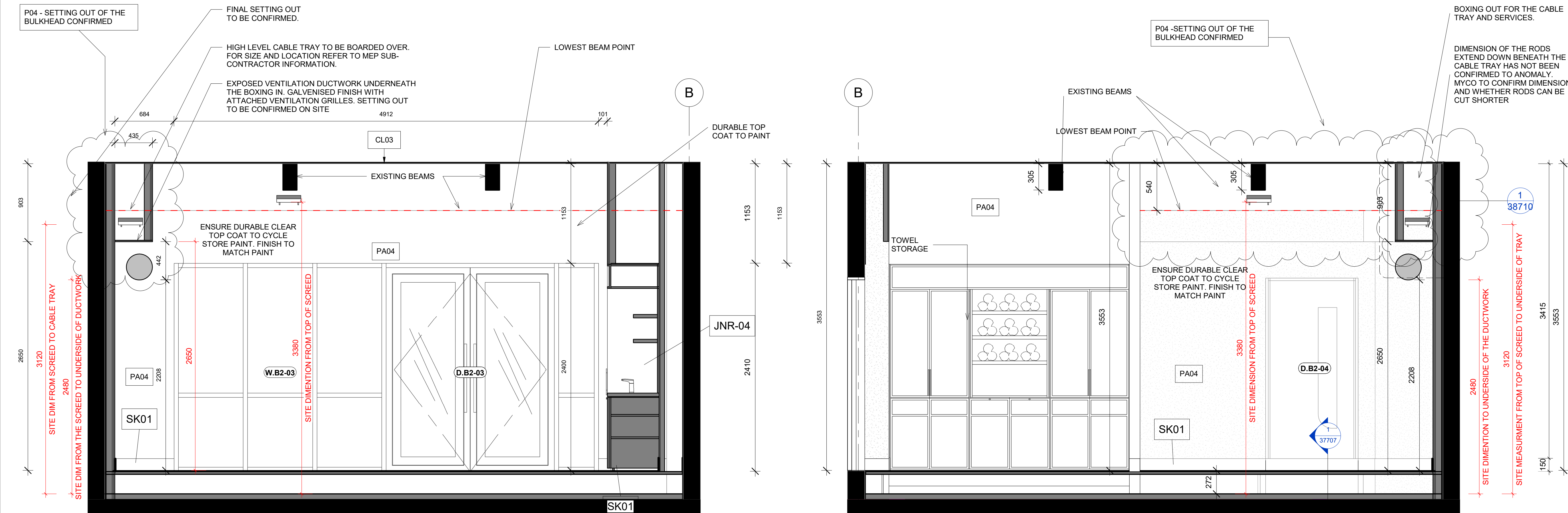
1 PROPOSED STUDIO ELEVATION A 1 : 25
