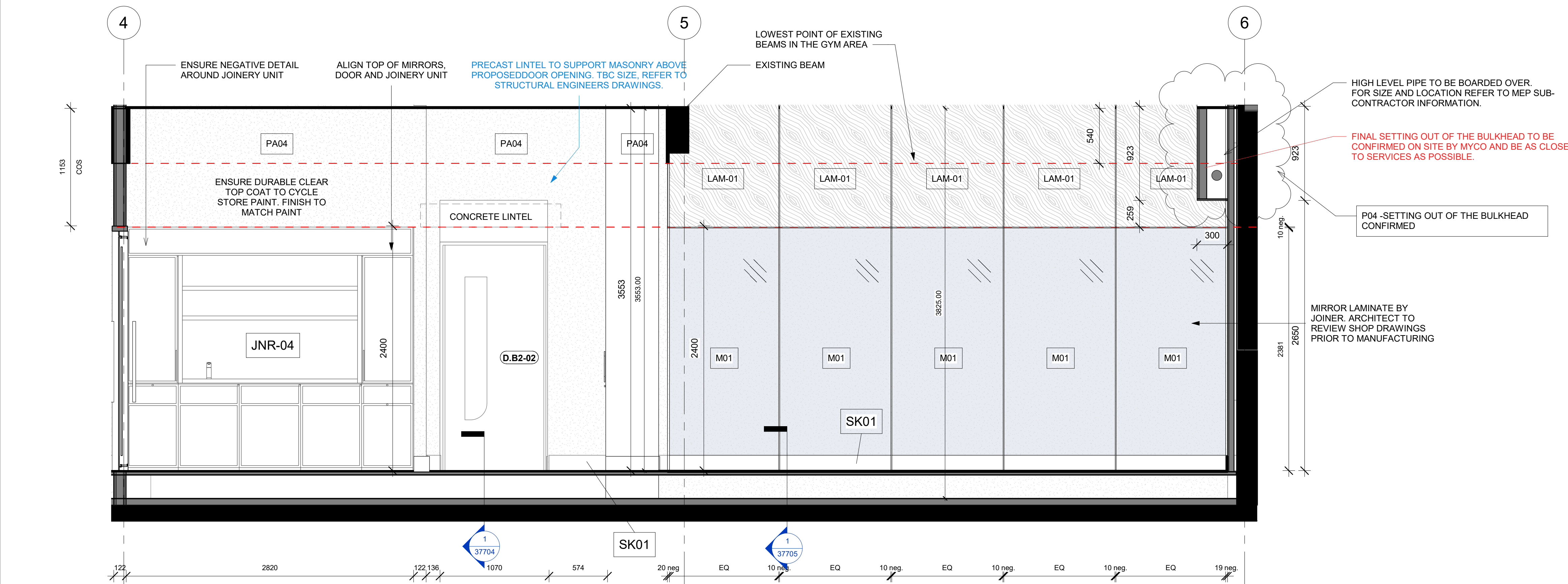
1 PROPOSED STUDIO ELEVATION A 1 : 25
