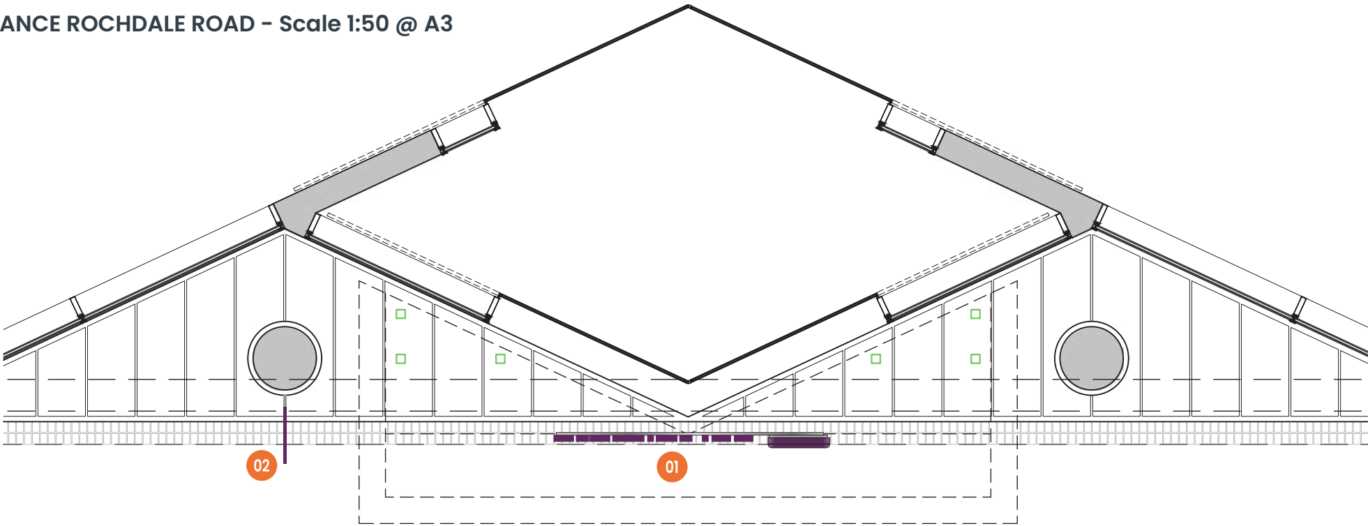
PLAN – Scale 1:50 @ A3
