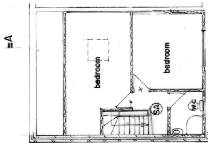
SECOND FLOOR PLAN (PROPOSED)
