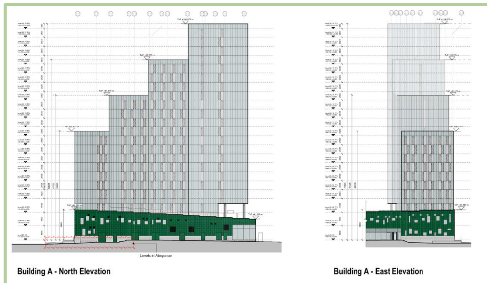
Figure 2.8 – North and East Elevation Block A
