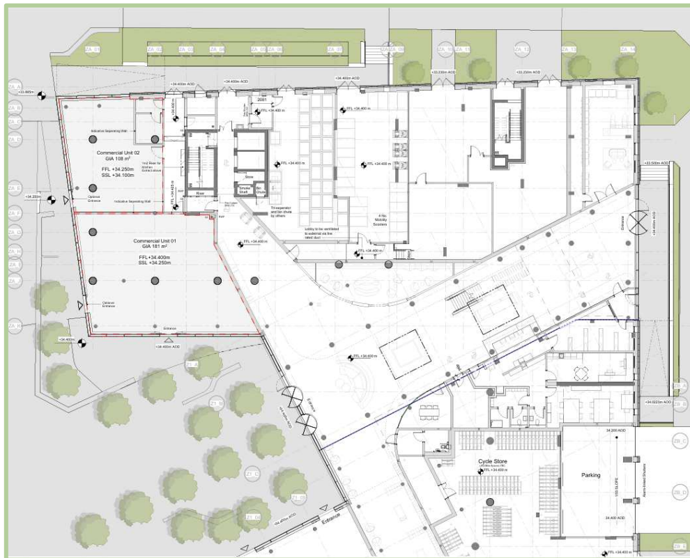
Figure 2.3 – Blocks A and B Ground Floor Podium Layout 2 of 2
