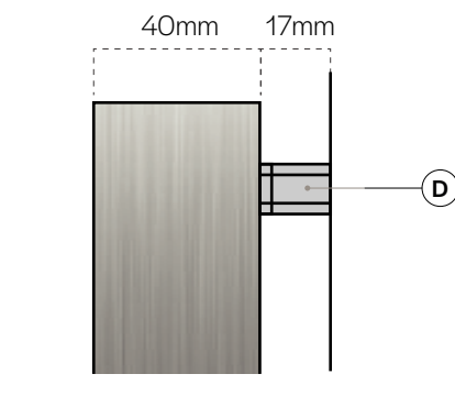
Side Detail - Letter Scale 1:2 @ A3
