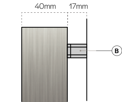
Side Detail Scale 1:2 @ A3
