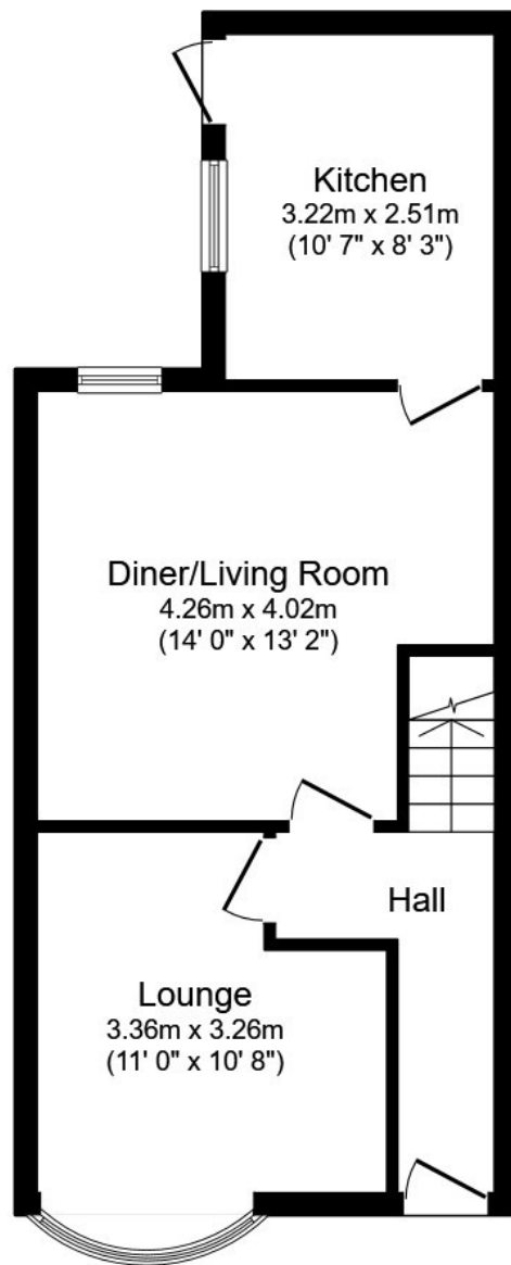
Ground Floor
