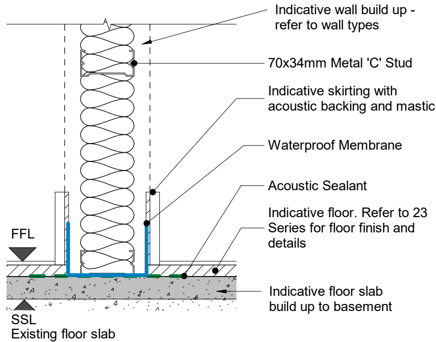
Typical Base Detail 1 : 5
