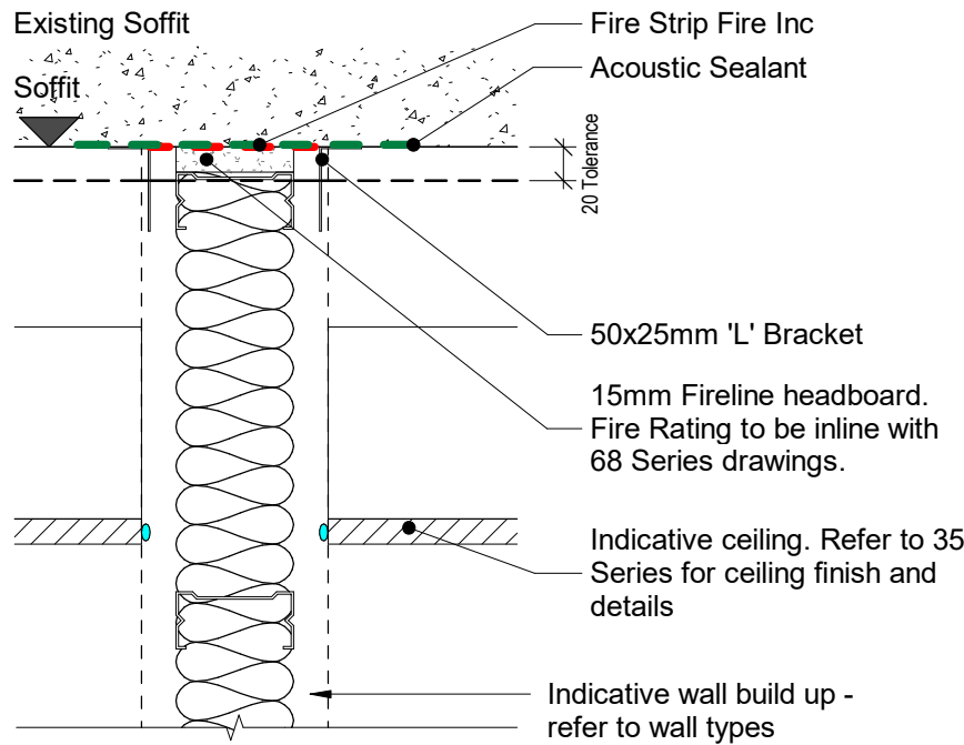
Typical Head Detail 1 : 5
