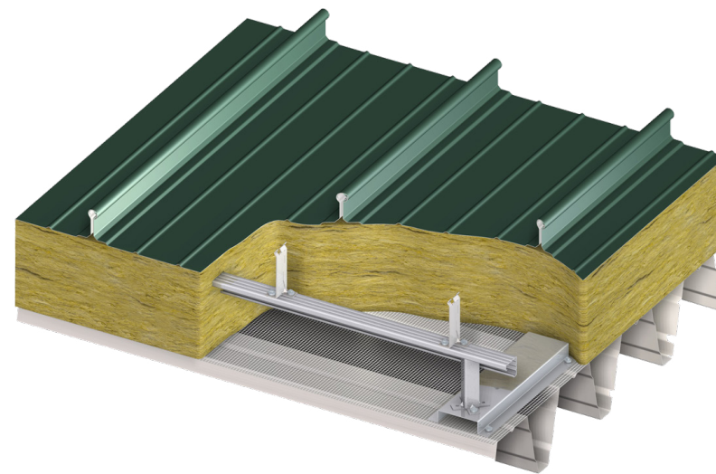
euroclad elite 5 roofing system
