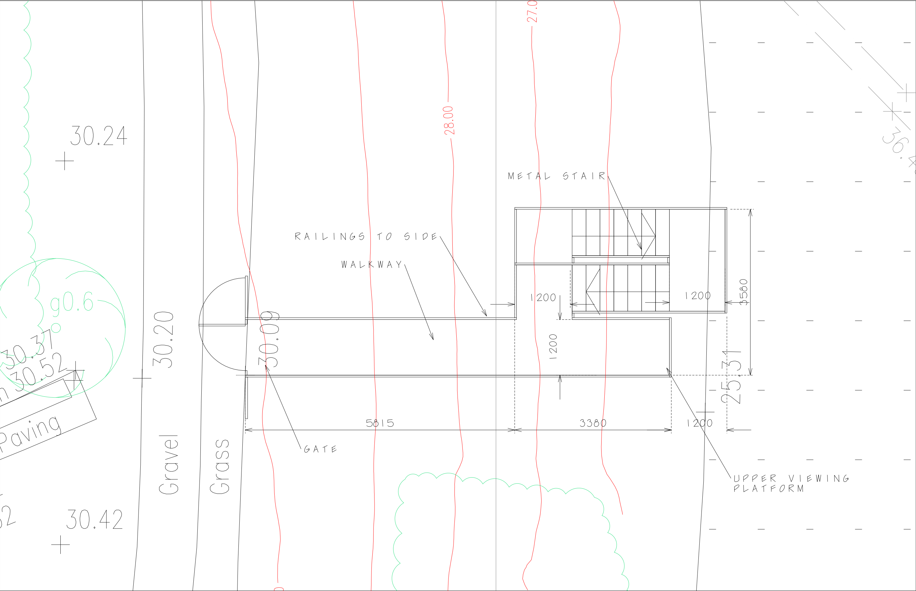
Access - footpath level plan
