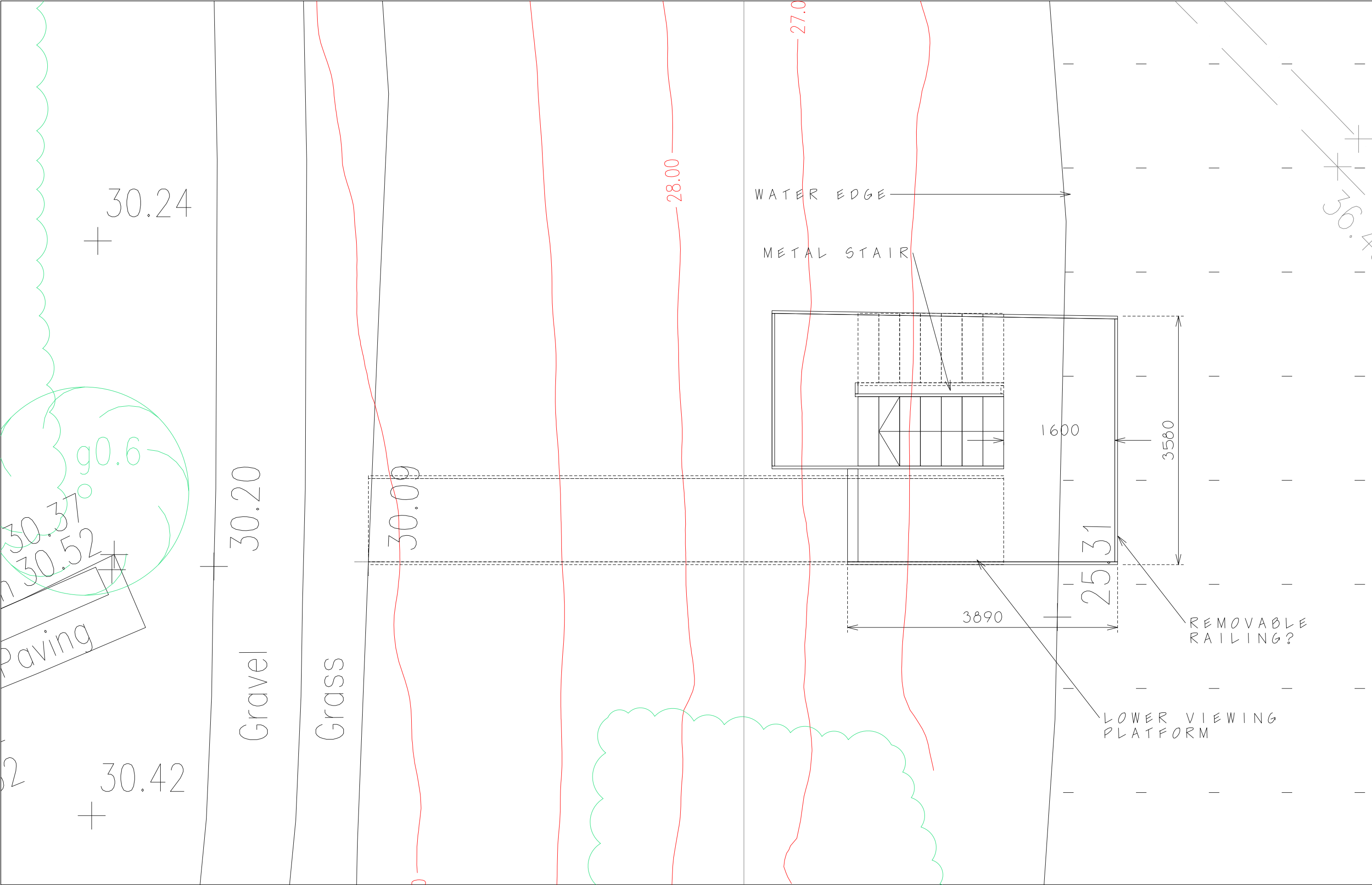
Jetty - lower level plan
