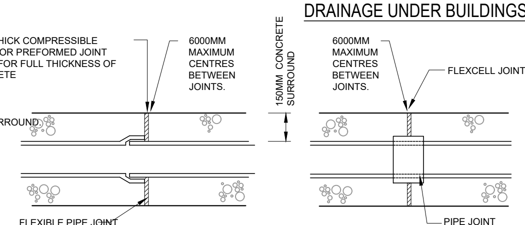
EXPANSION JOINT FOR CONCRETE BED AND SURROUND (SCALE 1:20)
