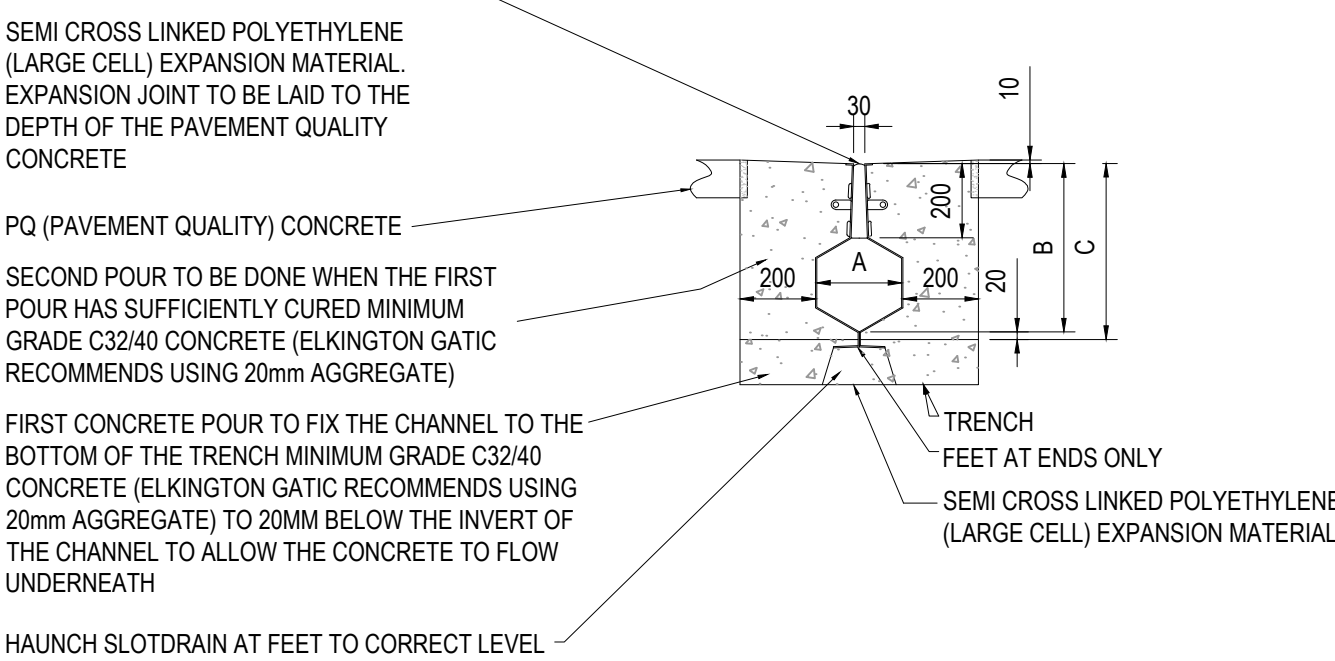
GATIC CASTSLOT TRESSAFE CONCRETE INSTALLATION
