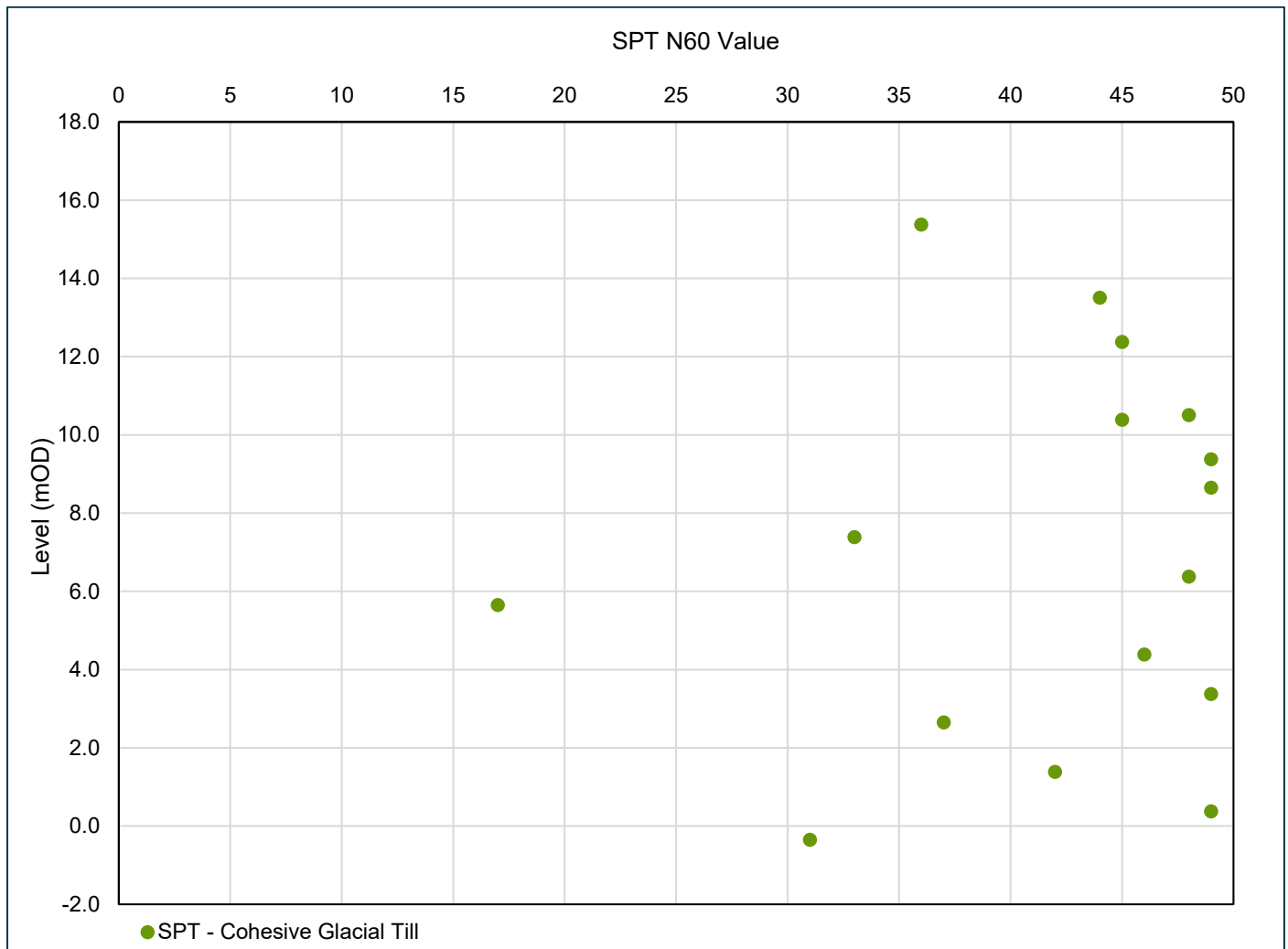
Plate 8: SPT N60 versus Level (mOD) – Glacial Till Deposits
