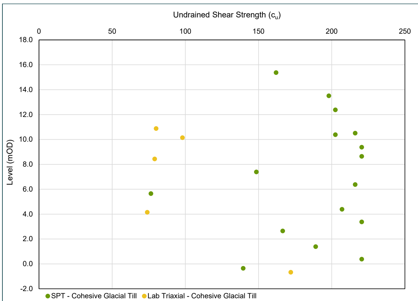
Plate 9: Undrained Shear Strength versus Level (mOD) – Glacial Till Deposits
