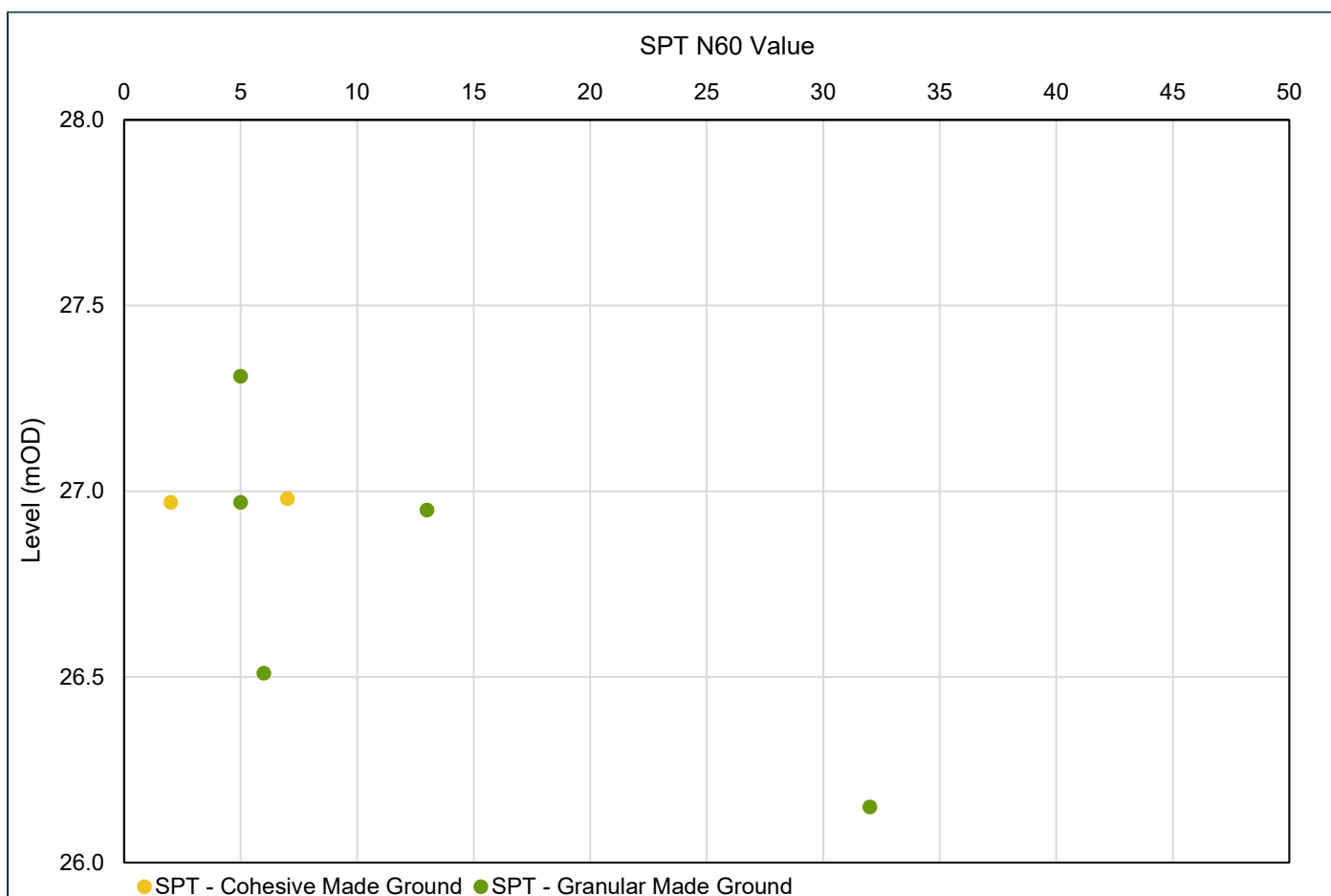
Plate 4: SPT N60 versus Level (mOD) – Made Ground
