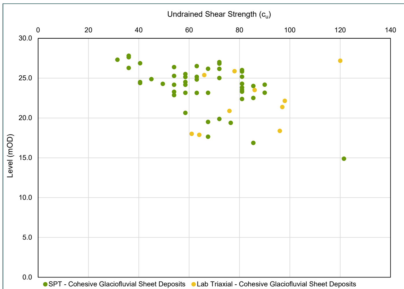
Plate 6: Undrained Shear Strength versus Level (mOD) – Cohesive Glaciofluvial Sheet Deposits
