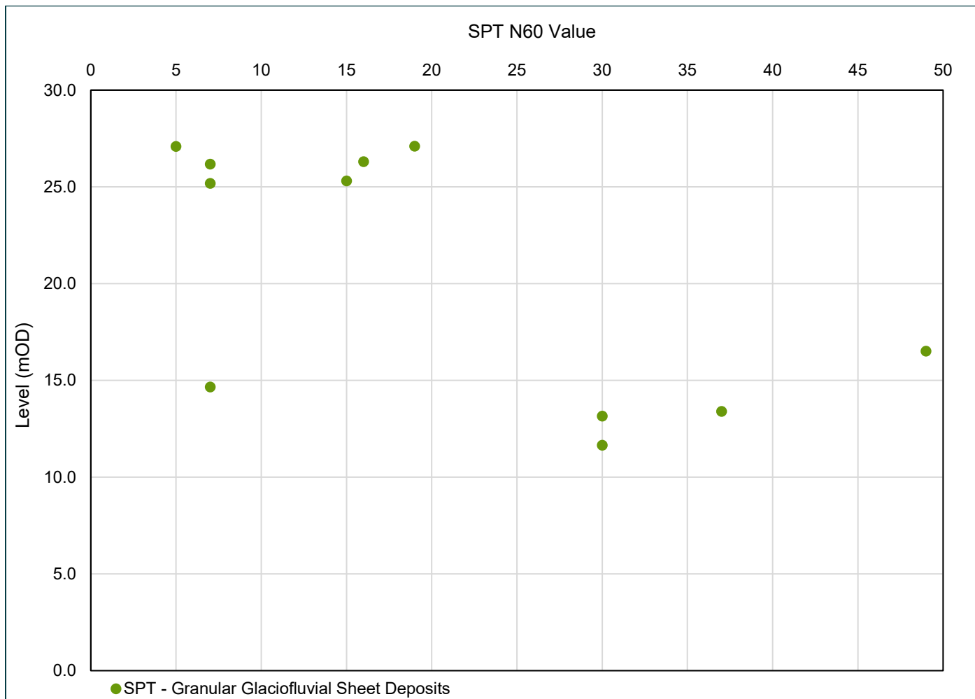
Plate 7: SPT N60 versus Level (mOD) – Granular Glaciofluvial Sheet Deposits
