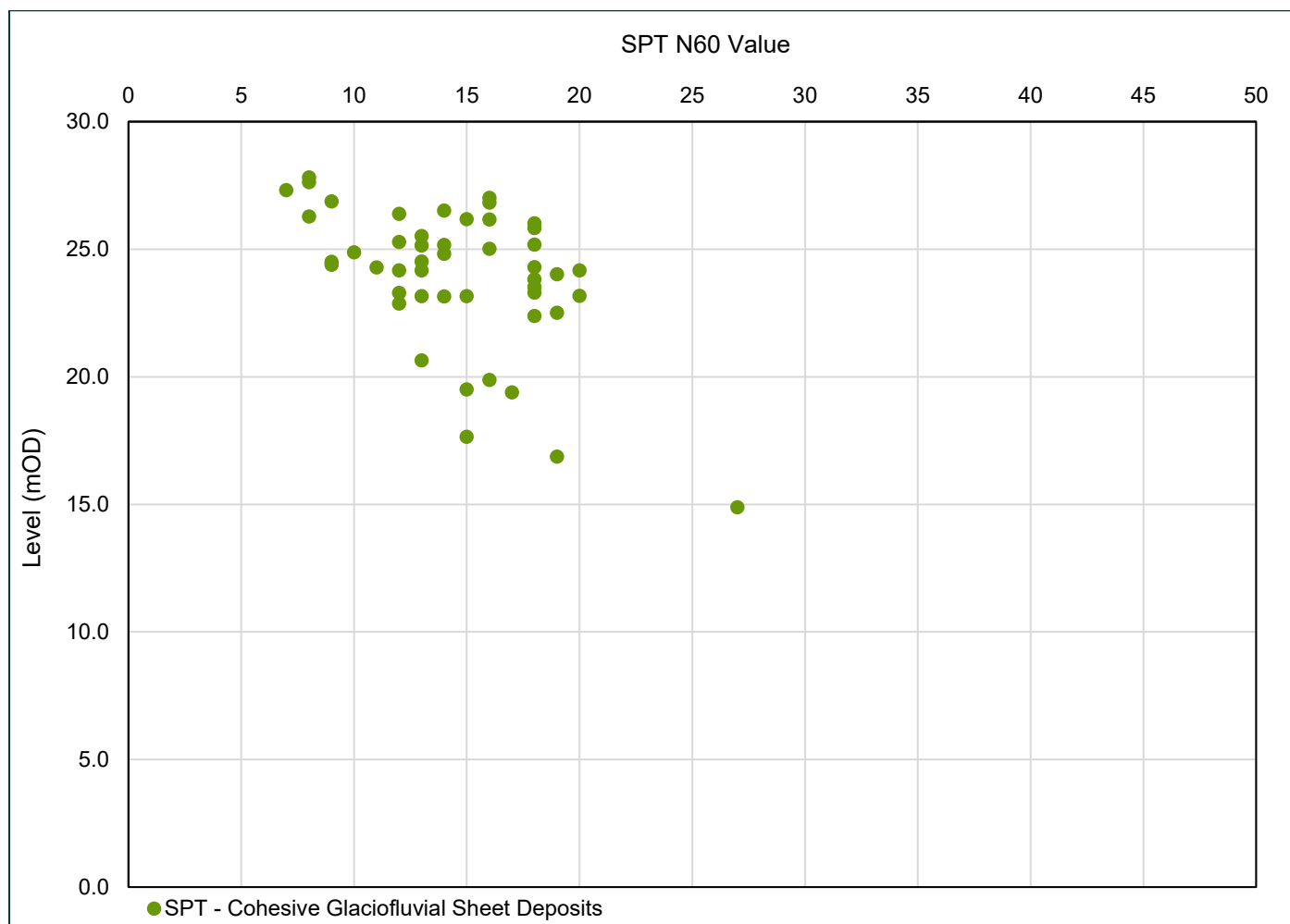
Plate 5: SPT N60 versus Level (mOD) – Cohesive Glaciofluvial Sheet Deposits
