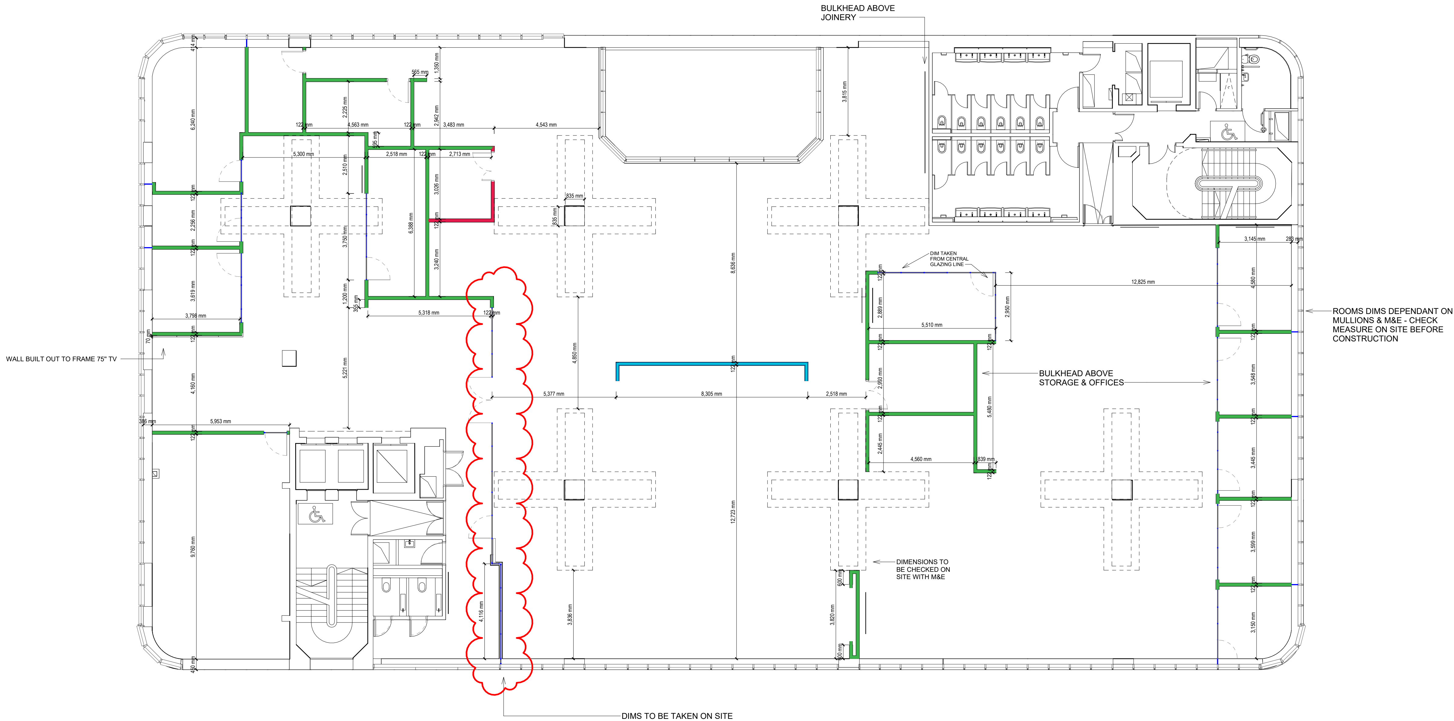
Setting out Plan - Level 04
