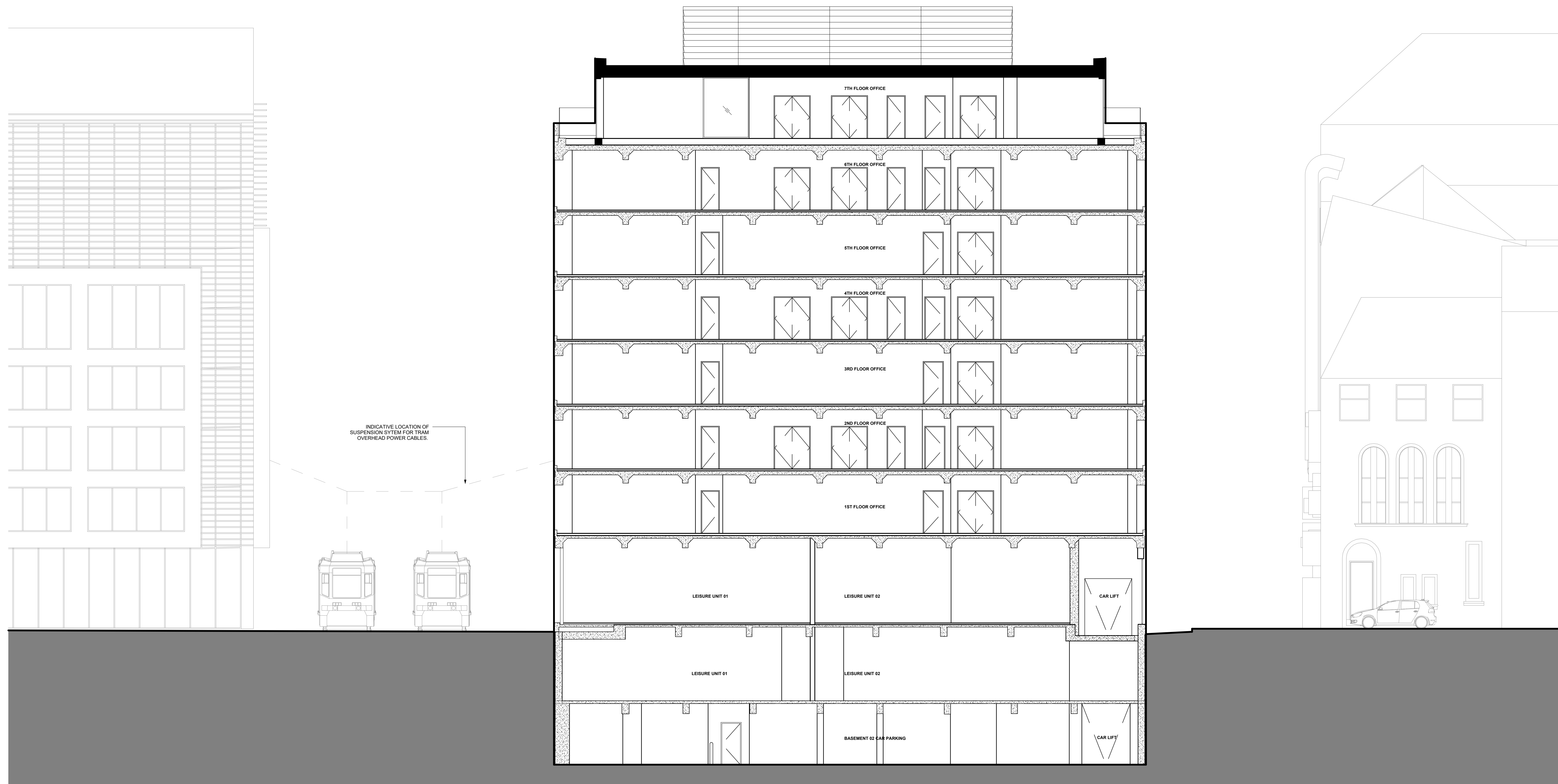
1 Existing Building Section 1 : 100
