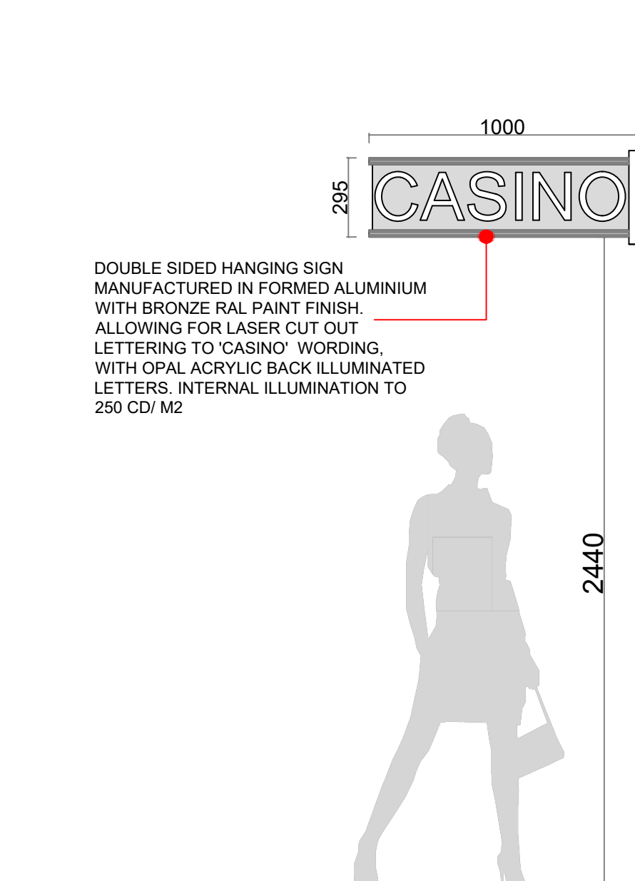
Oxford Street Proposed Hanging Sign Scale @ 1:20
