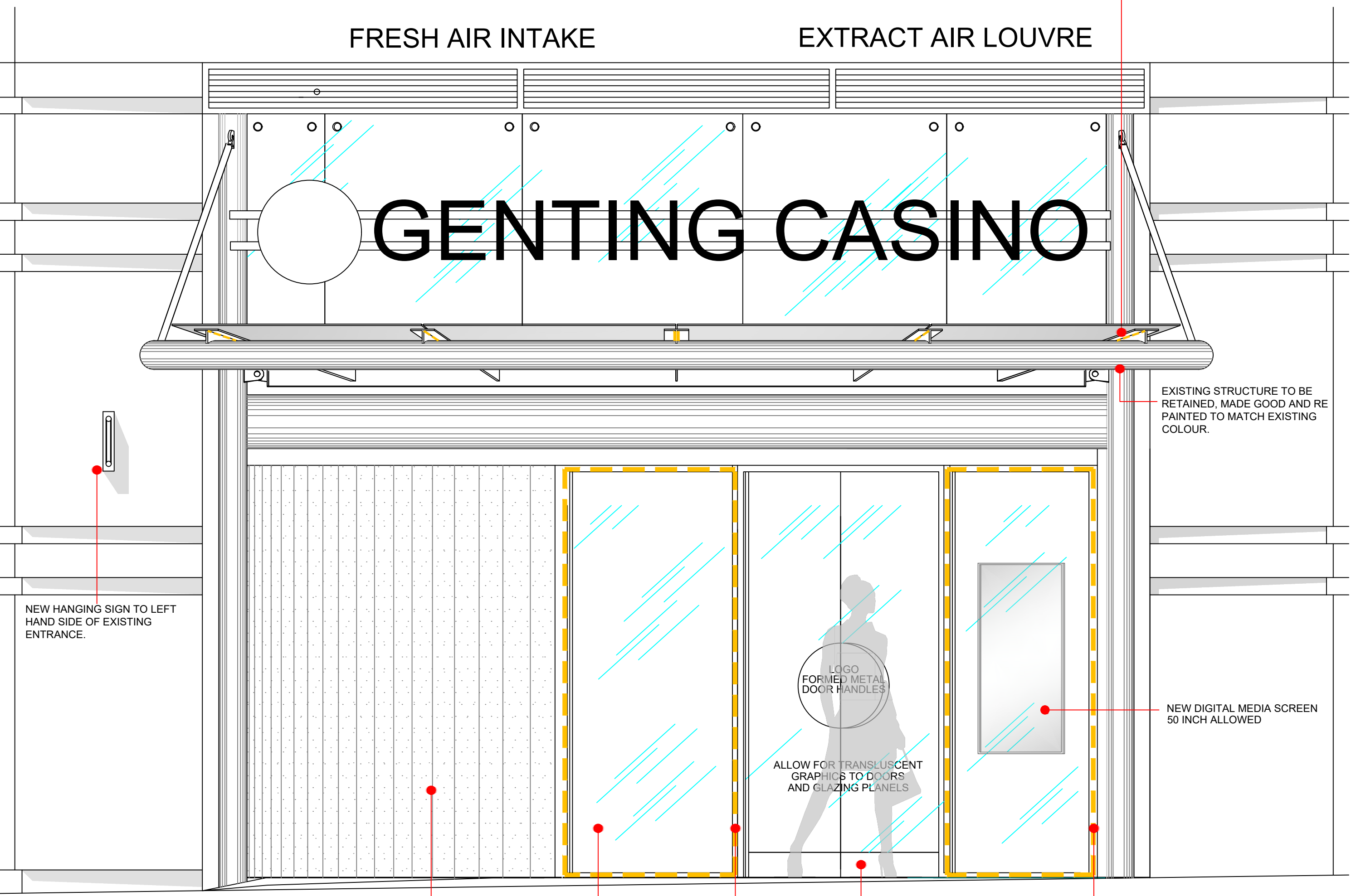
Proposed Entrance Elevation Scale @ 1:20
