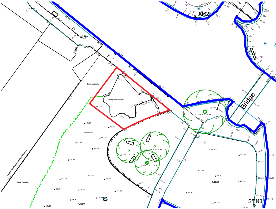
Existing Block Plan - Ancillary Building
