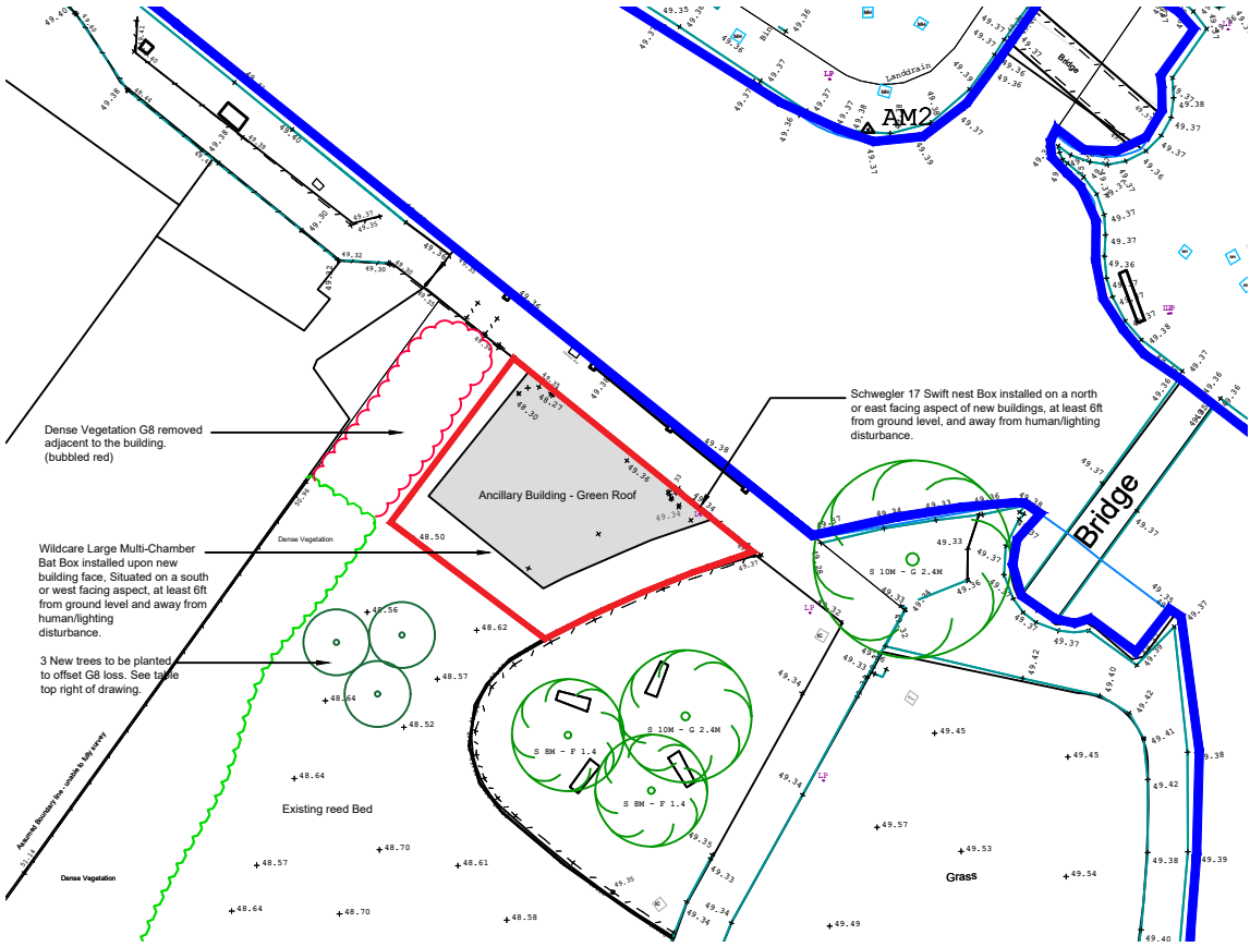
Proposed Block Plan - Ancillary Building
