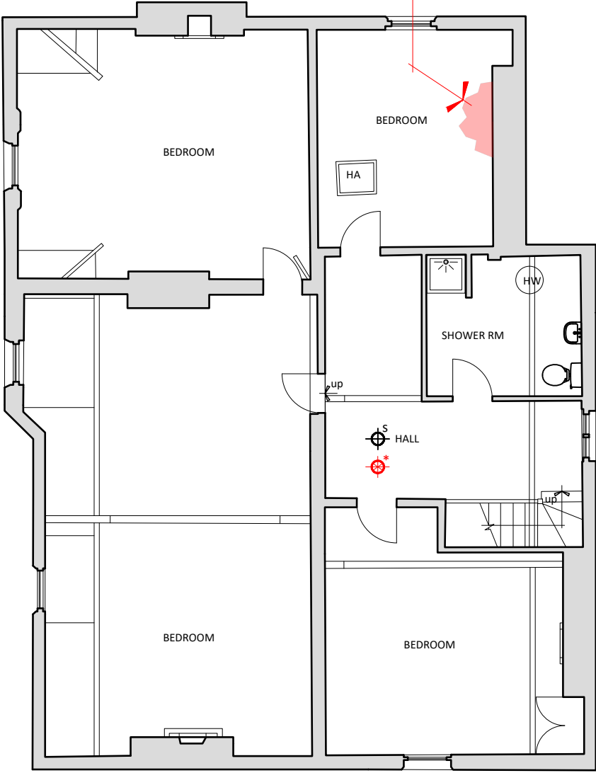
Second Floor Plan (1 to 100 @ A3)
