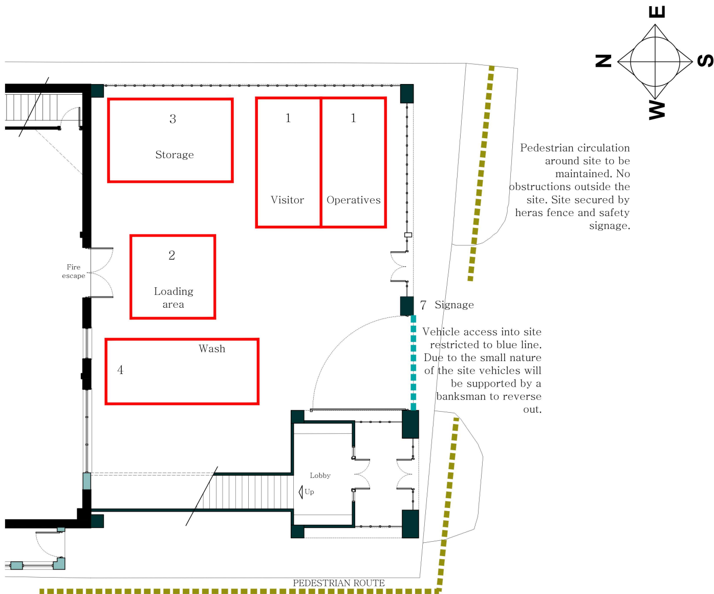
PROPOSED SITE PLAN (UNDERCROFT)
