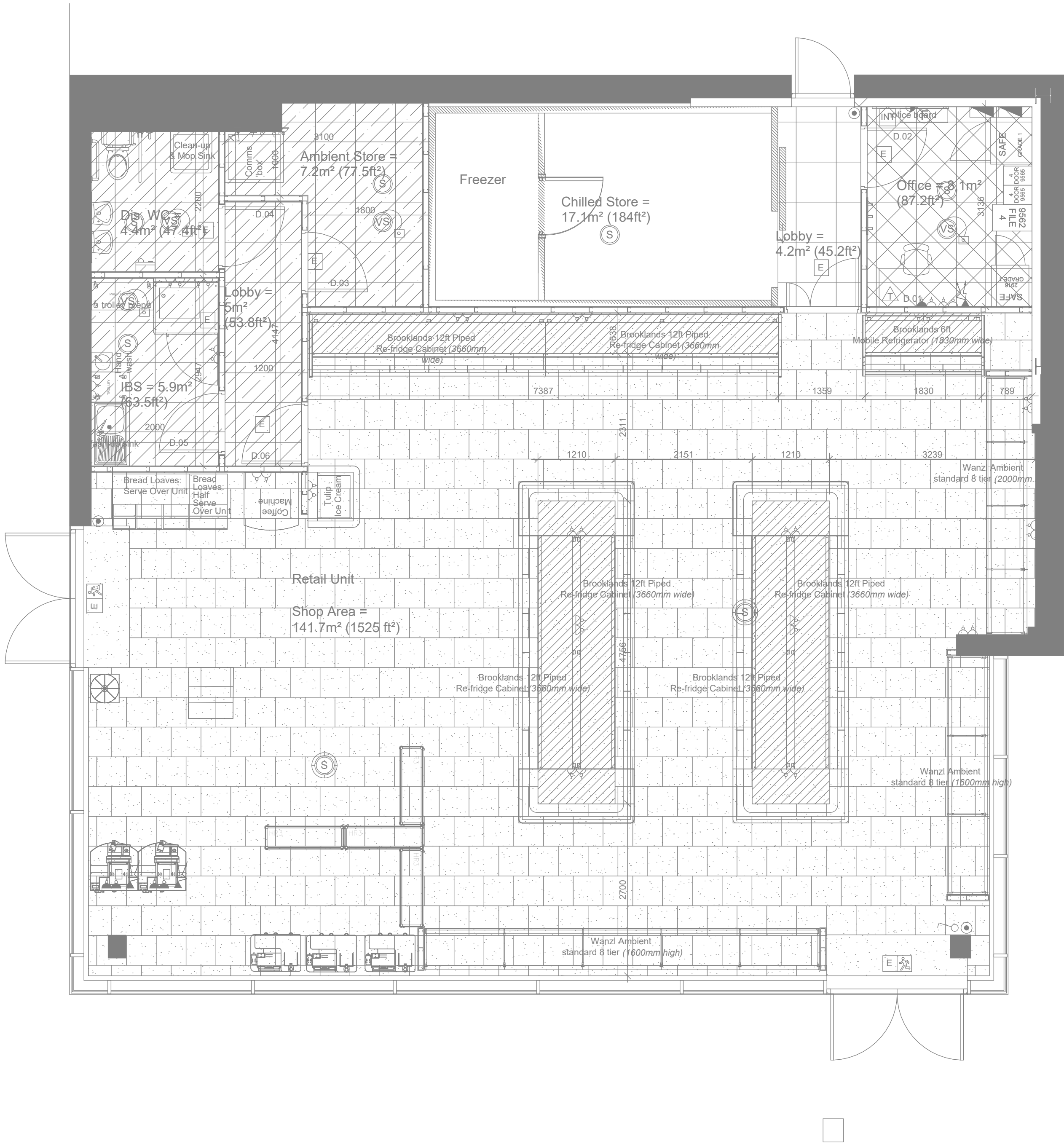
EXISTING GROUND FLOOR 1 : 50
