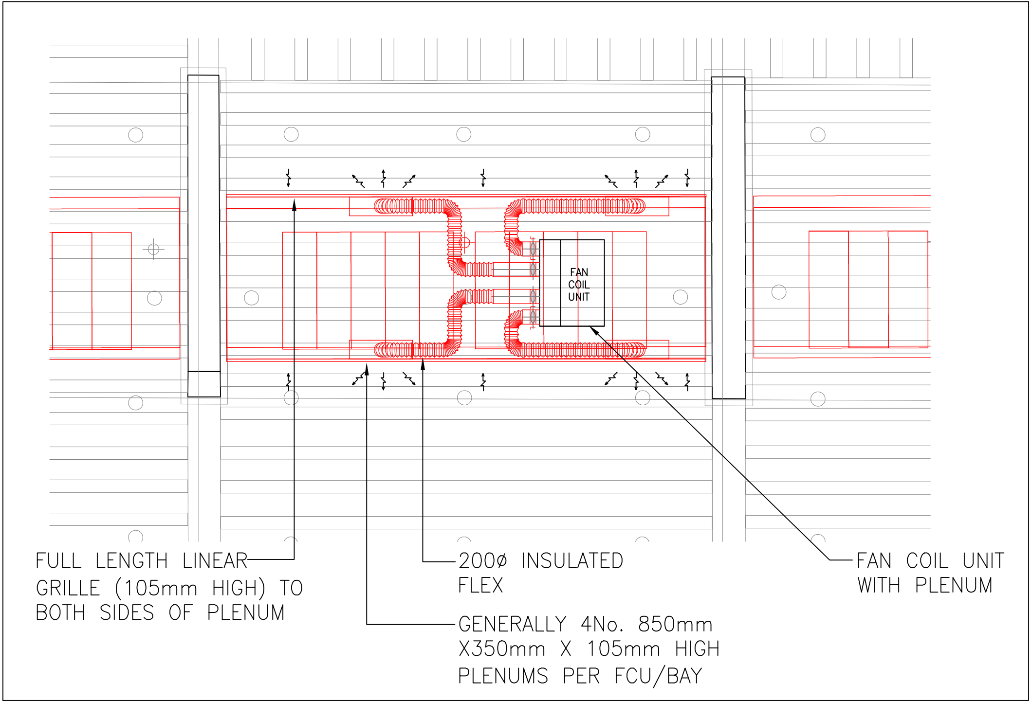
TYPICAL FAN COIL UNIT RAFT DETAIL
