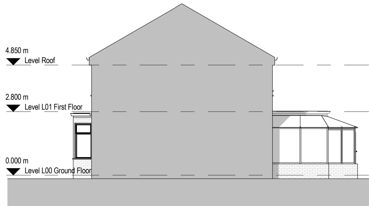
4 Existing West Elevation 1 : 100
