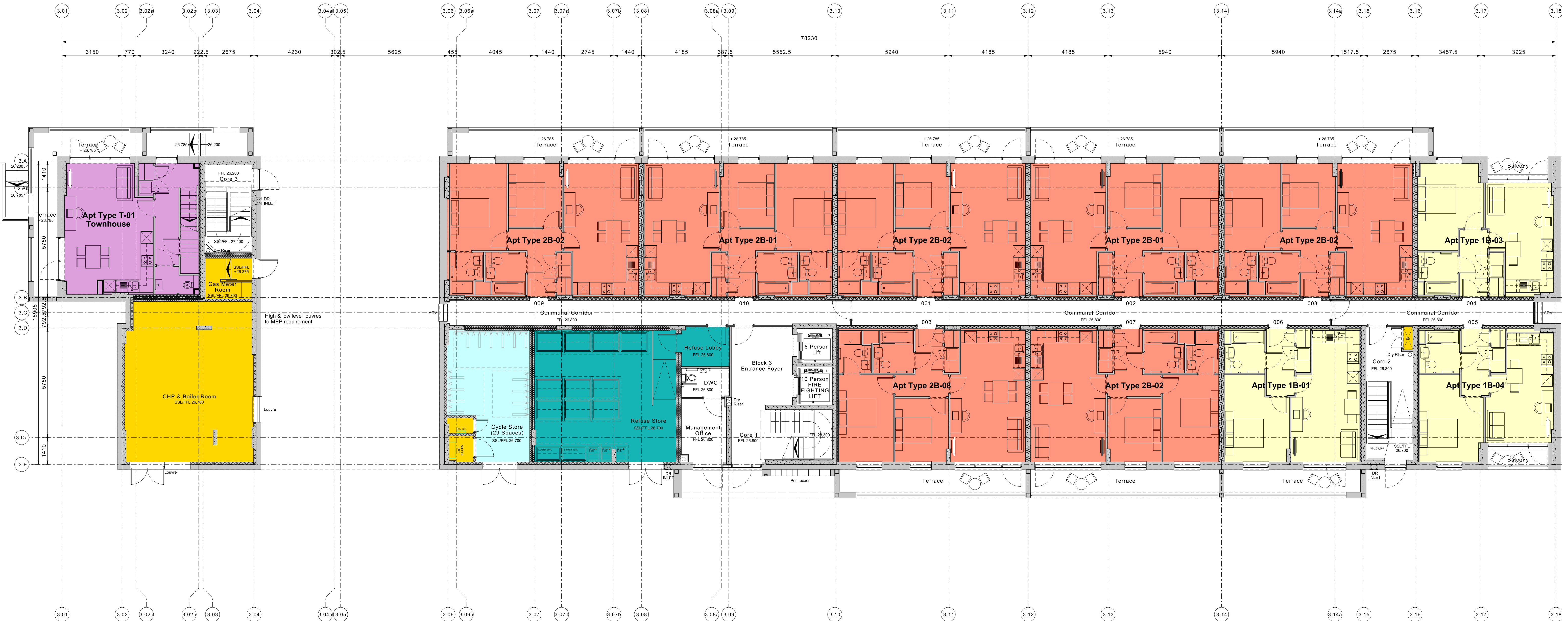
P3010.01 Block 3 - Ground Floor (Level 0) GA Plan 1:100@A1
