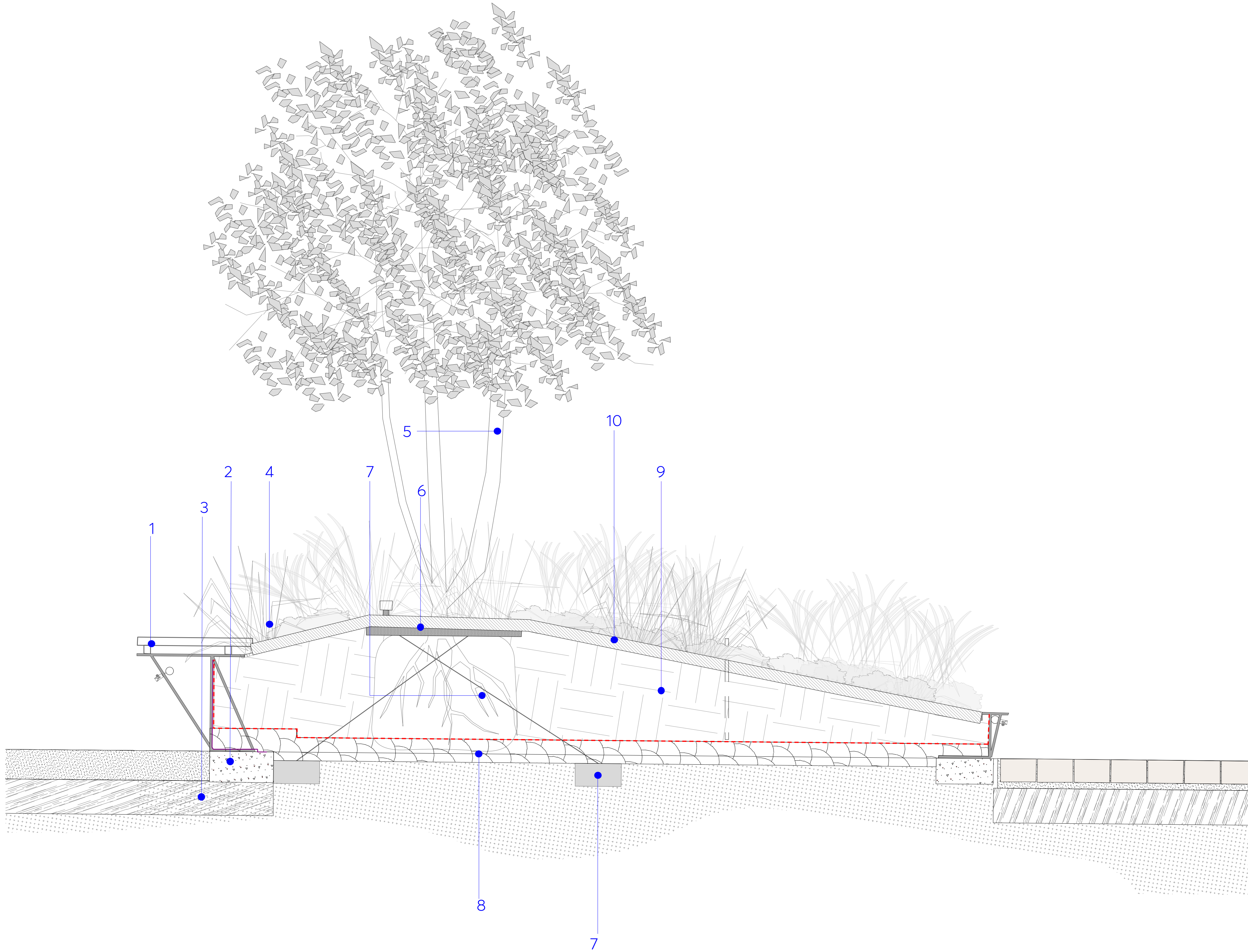
TREE TYPICAL SECTION CONTECTION SCALE 1:10
