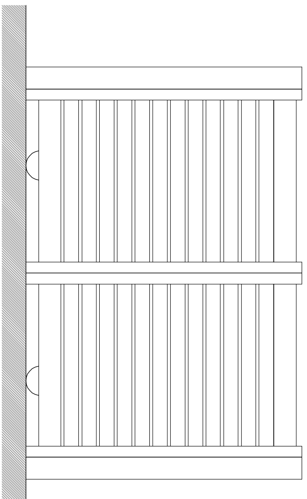
New Bin Store Elevation 1
