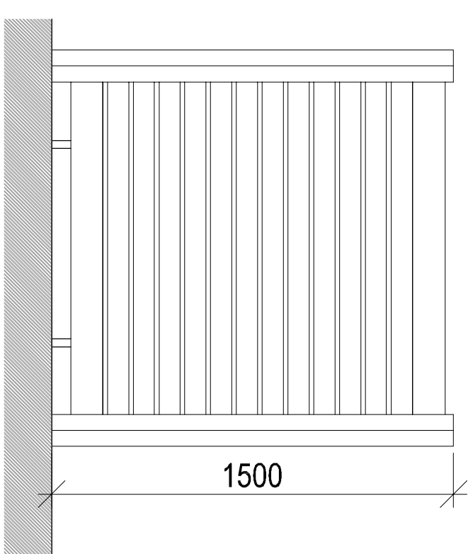
New Bin Store Elevation 02
