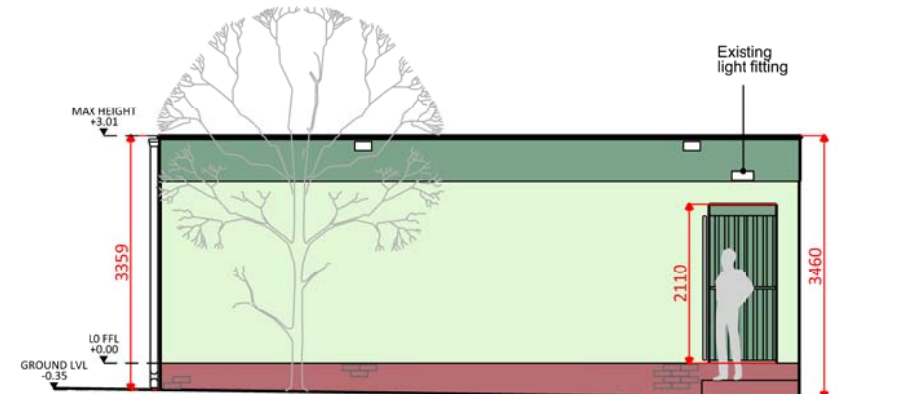
03 EXISTING TEMPORARY BUILDING WEST ELEVATION
