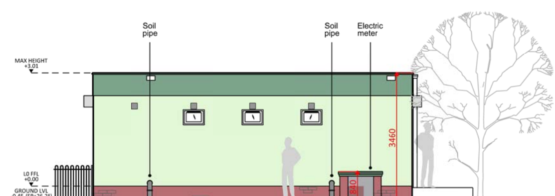
04 EXISTING TEMPORARY BUILDING EAST ELEVATION
