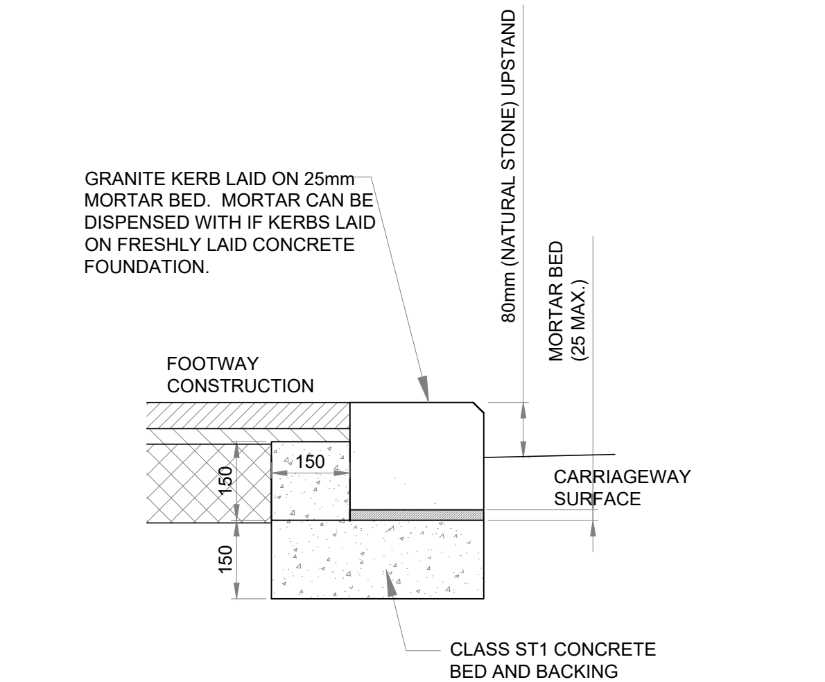
UPSTAND KERB SCALE 1:10
