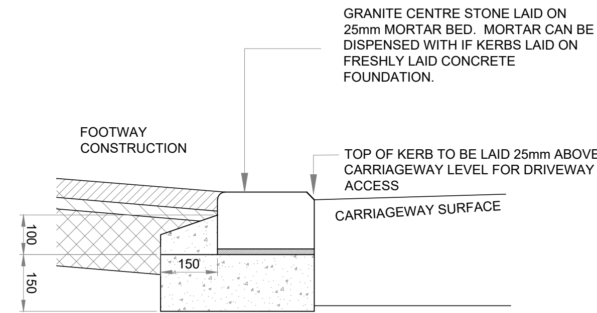
UPSTAND KERB SCALE 1:10
