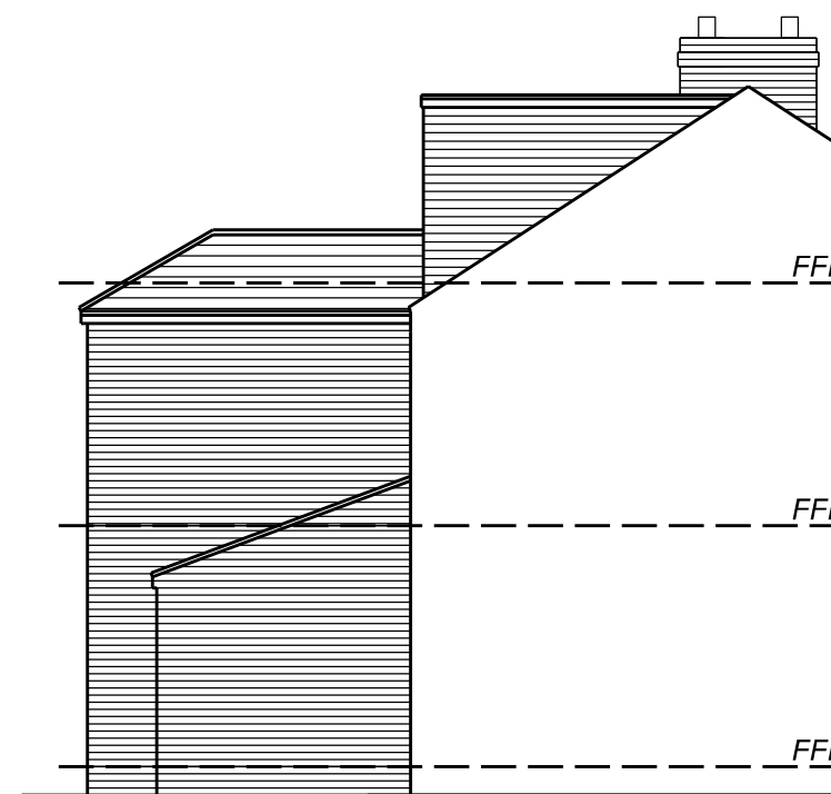
North Elevation
