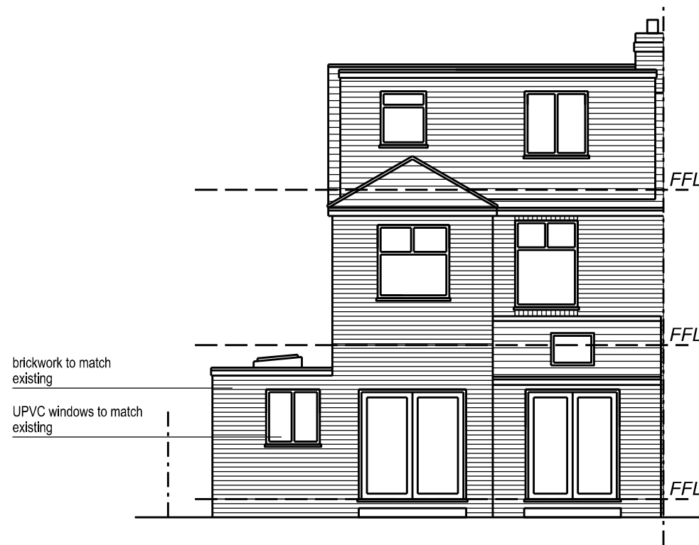
East Elevation
